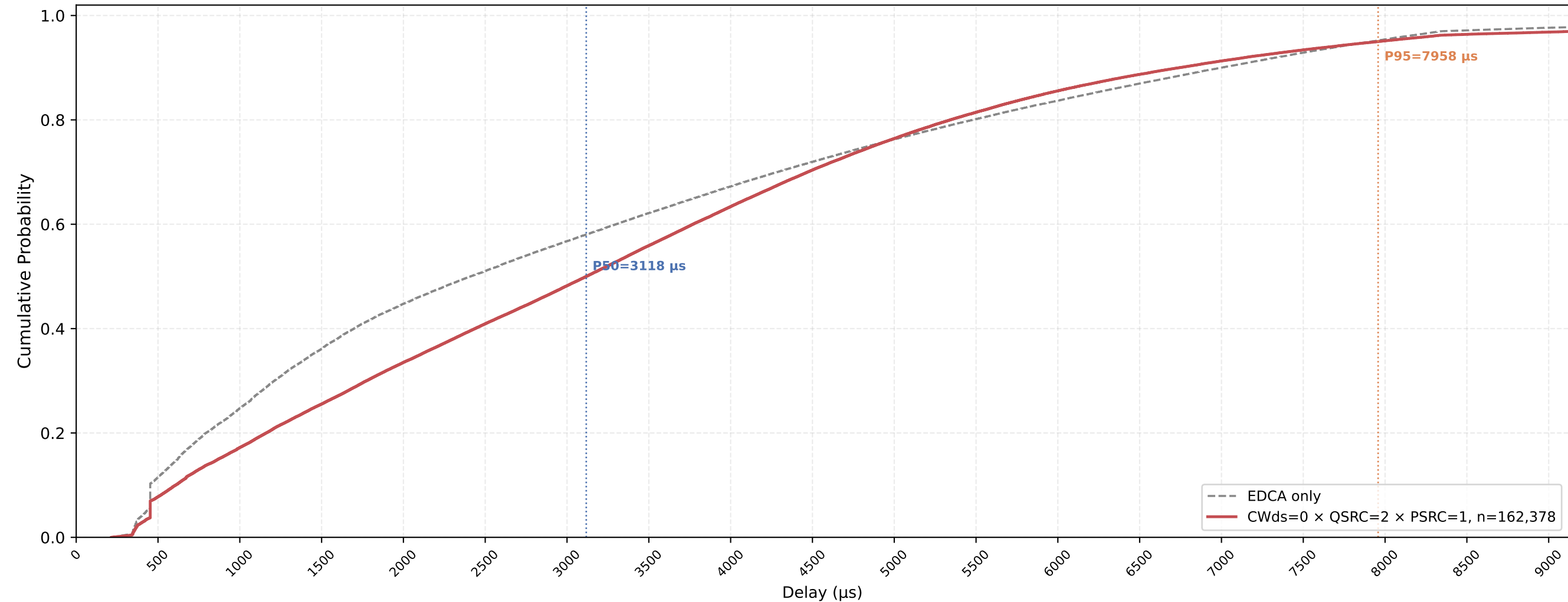
P-EDCA STA VO Delay CDF — CWds=0 × QSRC=2 × PSRC=1 nSta=30, nPedca=30, 1Mbps, avg of 10 runs
