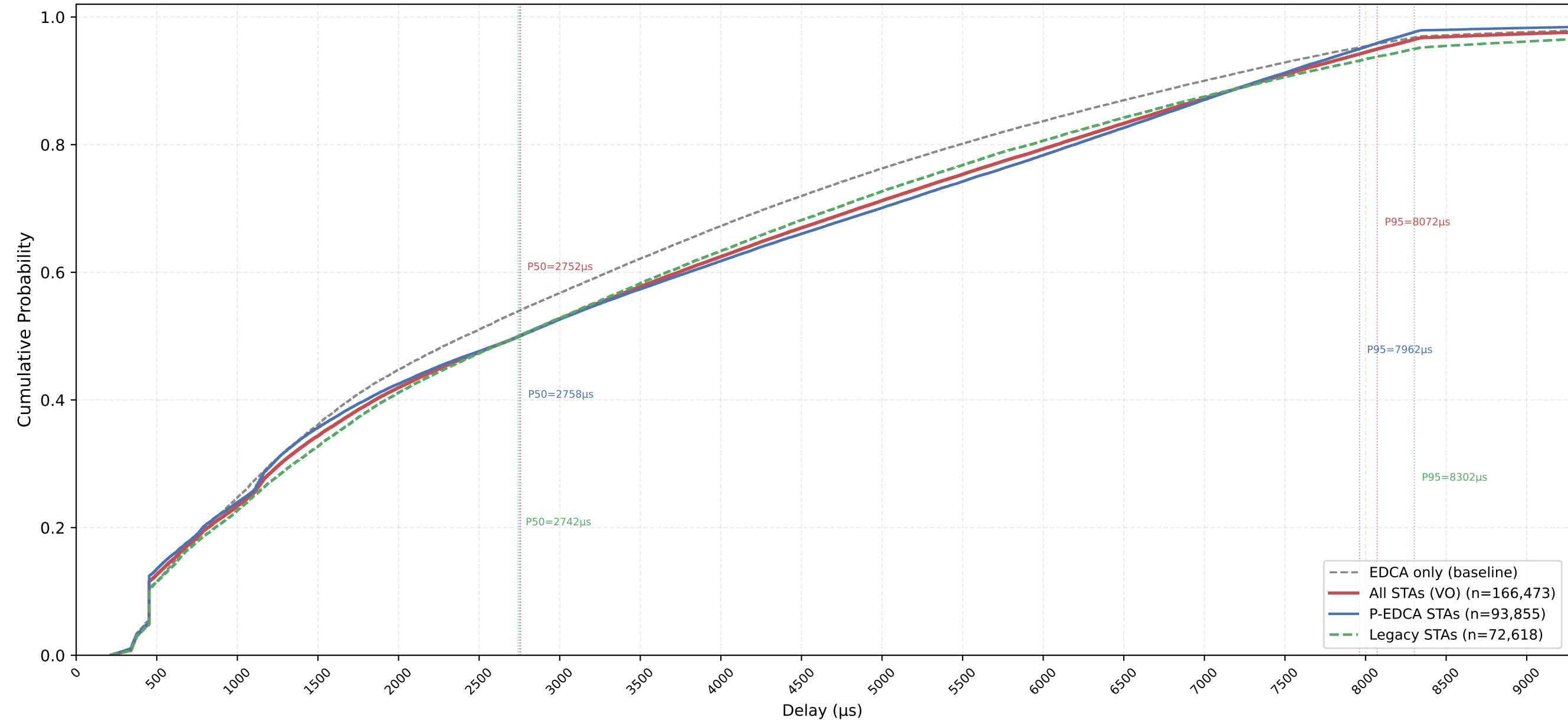
VO Delay CDF — P-EDCA / Legacy / All | CWds=0 × QSRC=4 × PSRC=1 nSta=30, nPedca=15/30, 1Mbps, avg of 10 runs
