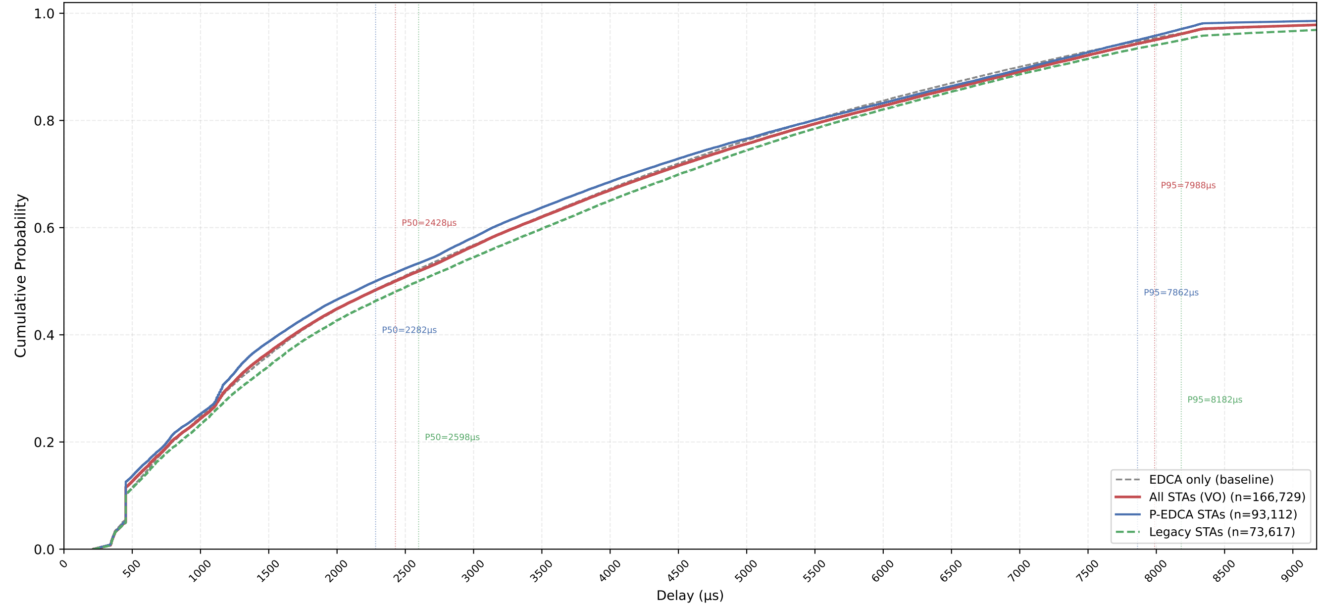
VO Delay CDF — P-EDCA / Legacy / All | CWds=0 × QSRC=5 × PSRC=1 nSta=30, nPedca=15/30, 1Mbps, avg of 10 runs
