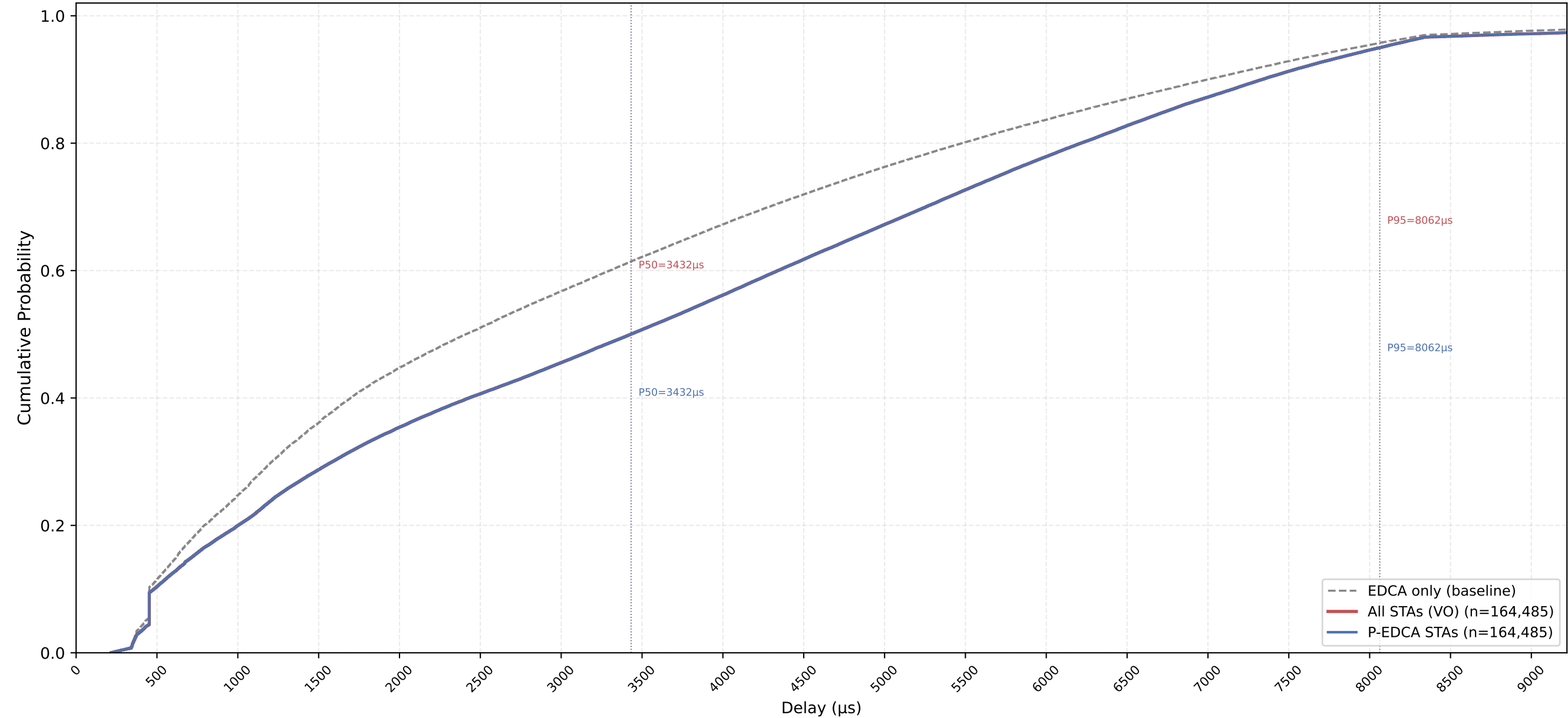
VO Delay CDF — P-EDCA / Legacy / All | CWds=1 × QSRC=3 × PSRC=1 nSta=30, nPedca=30/30, 1Mbps, avg of 10 runs
