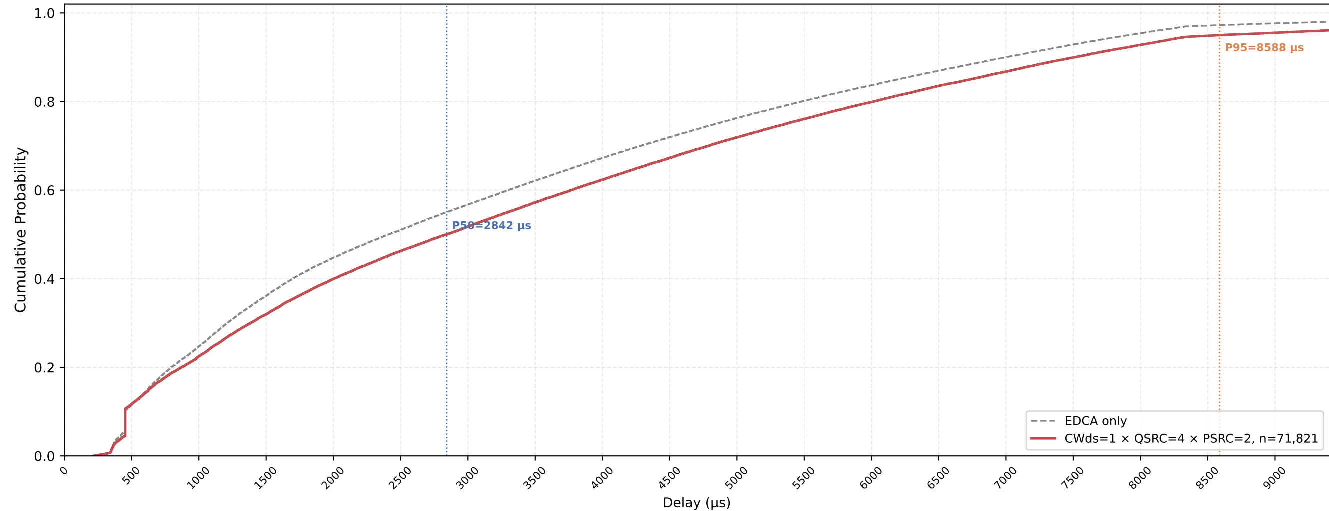
Legacy STA VO Delay CDF — CWds=1 × QSRC=4 × PSRC=2 nSta=30, nPedca=15, 1Mbps, avg of 10 runs
