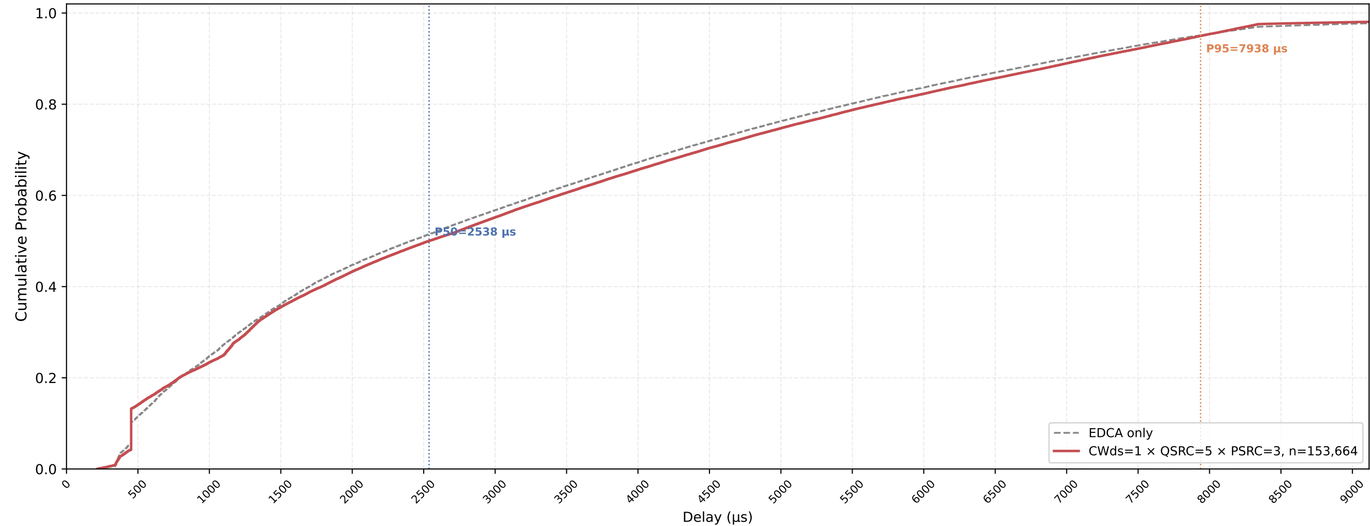
P-EDCA STA VO Delay CDF — CWds=1 × QSRC=5 × PSRC=3 nSta=30, nPedca=30, 1Mbps, avg of 10 runs
