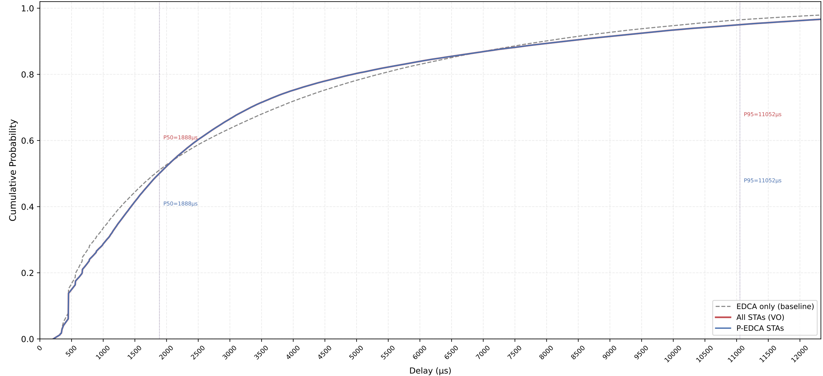
VO Delay CDF — P-EDCA / Legacy / All | CWds=0 × QSRC=1 × PSRC=3 nSta=30, nPedca=30/30, 1Mbps, avg of 10 runs
