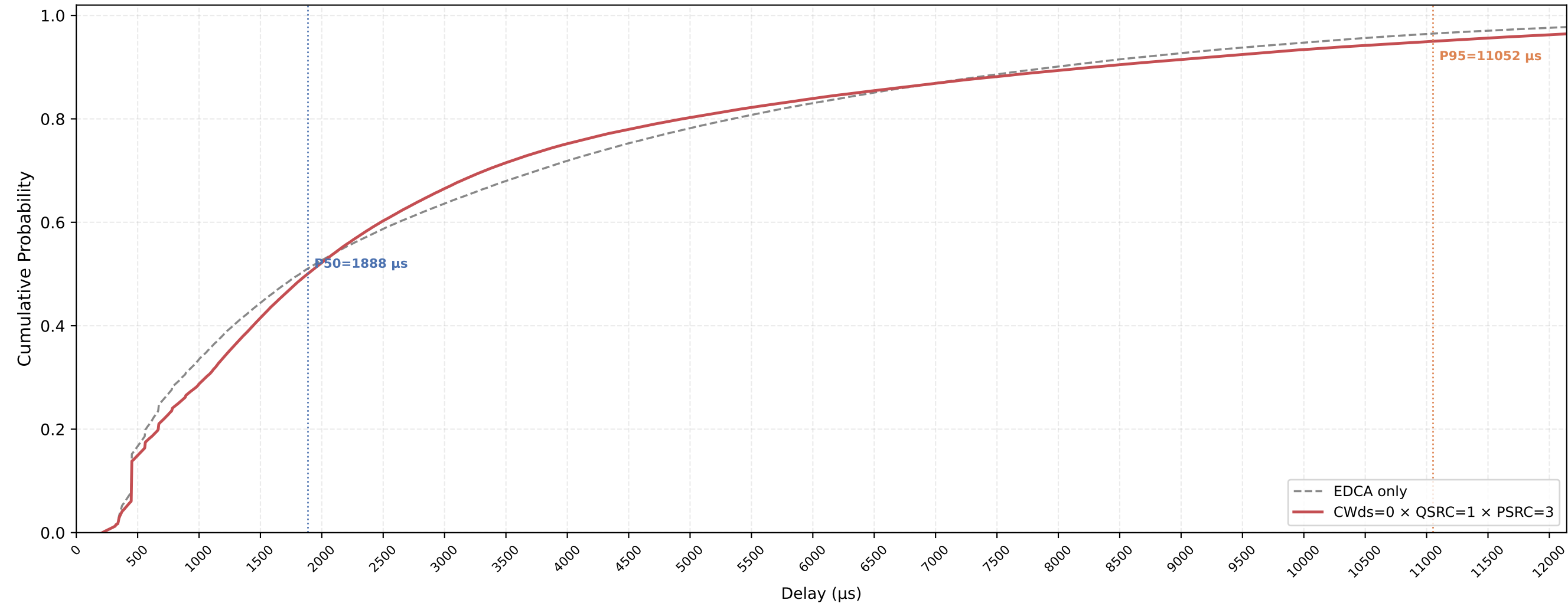
VO (all STAs) Delay CDF — CWds=0 × QSRC=1 × PSRC=3 nSta=30, nPedca=30, 1Mbps, avg of 10 runs
