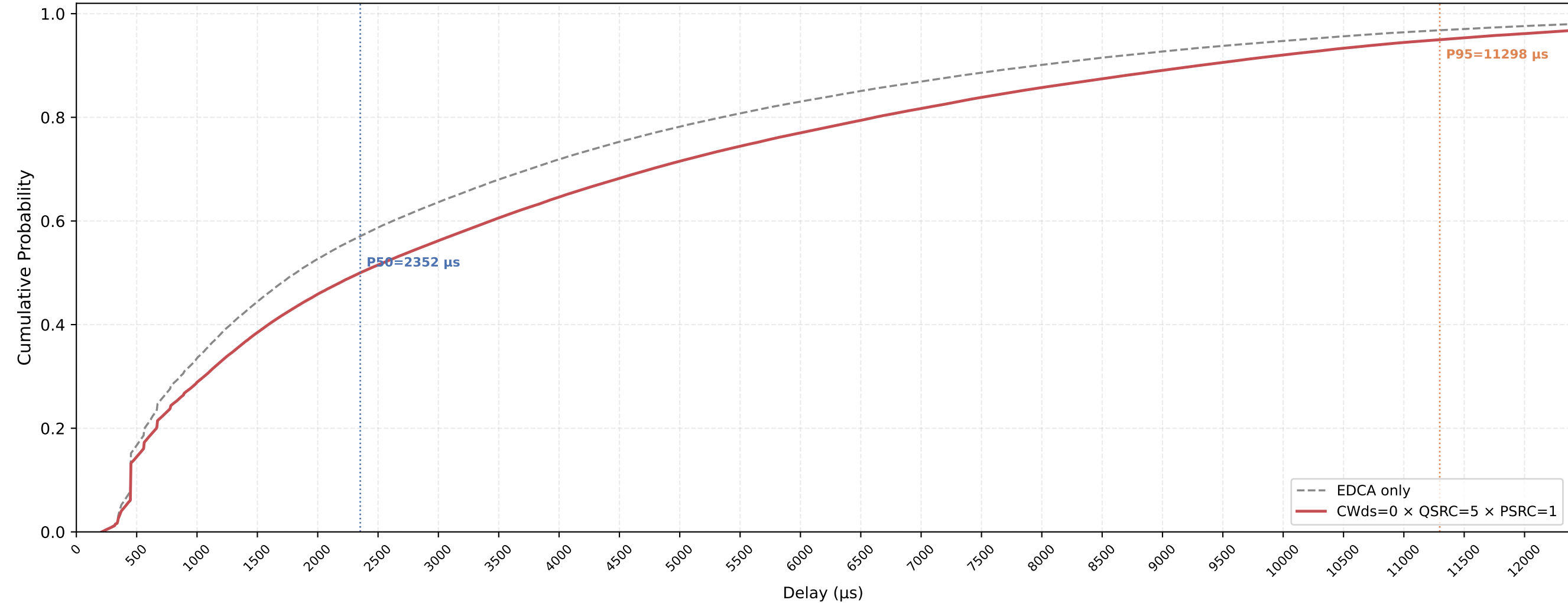
P-EDCA STA VO Delay CDF — CWds=0 × QSRC=5 × PSRC=1 nSta=30, nPedca=30, 1Mbps, avg of 10 runs
