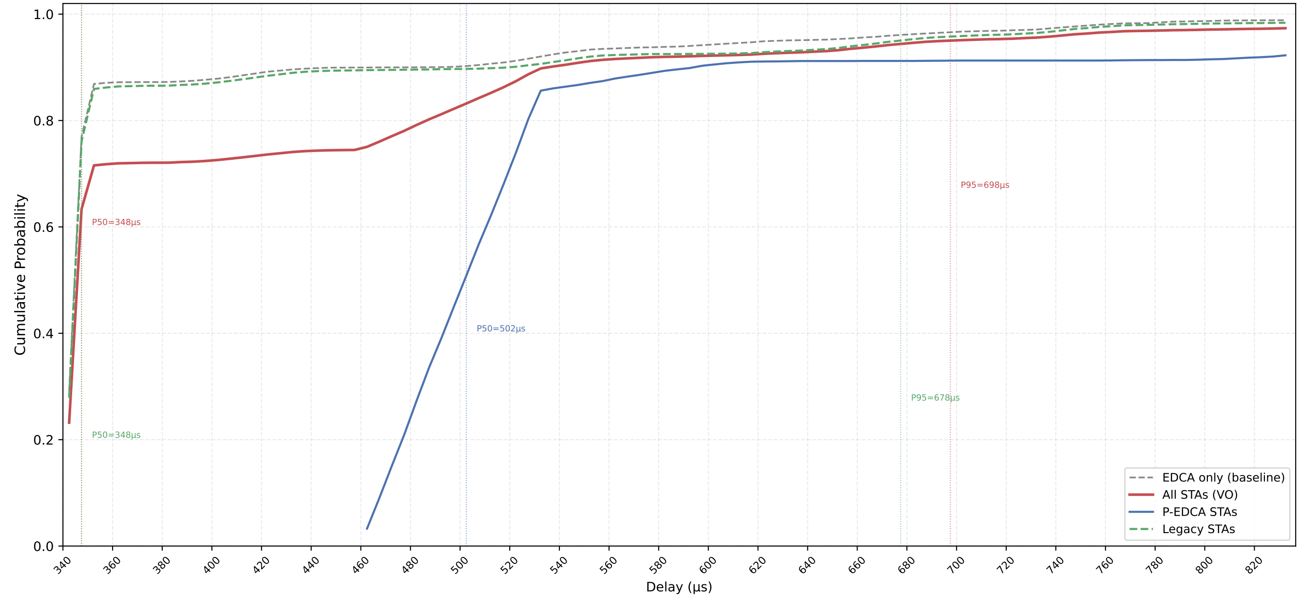
VO Delay CDF — P-EDCA / Legacy / All | CWds=0 × QSRC=0 × PSRC=1 nSta=30, nPedca=5/30, 0.1Mbps, avg of 10 runs
