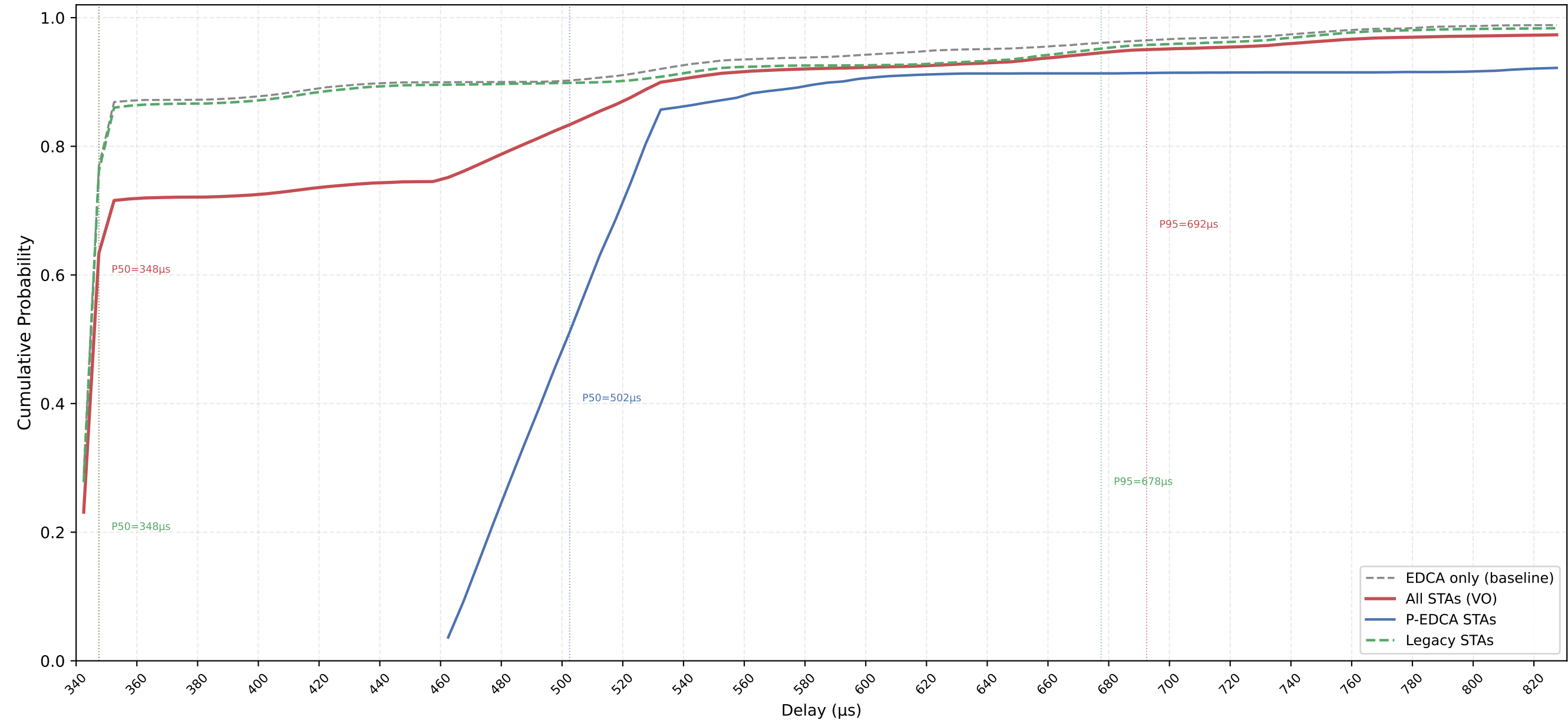
VO Delay CDF — P-EDCA / Legacy / All | CWds=0 × QSRC=0 × PSRC=2 nSta=30, nPedca=5/30, 0.1Mbps, avg of 10 runs
