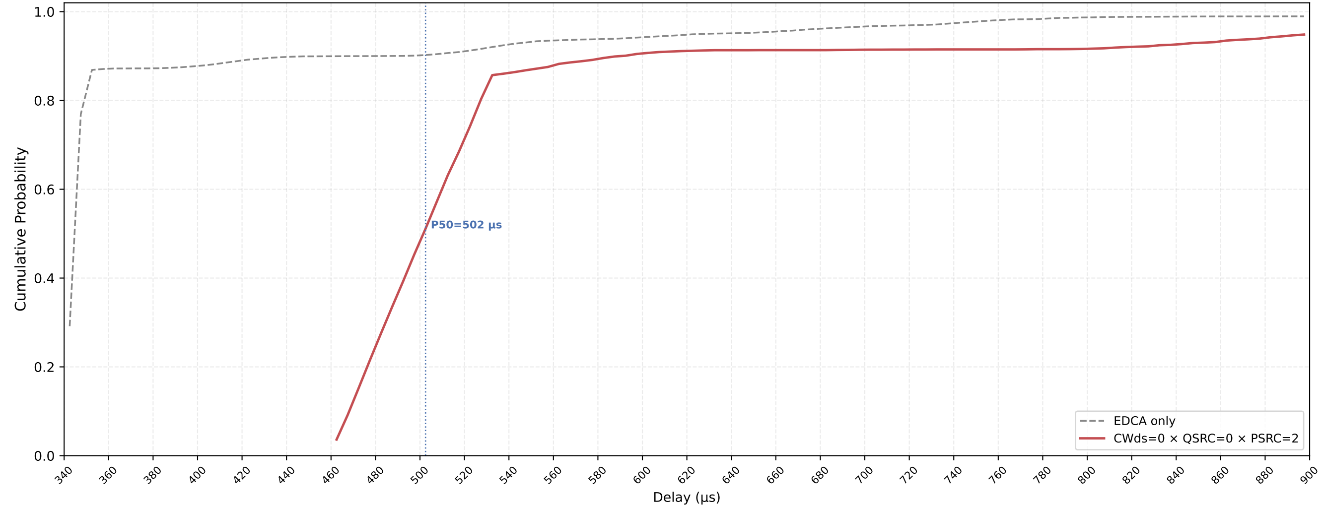
P-EDCA STA VO Delay CDF — CWds=0 × QSRC=0 × PSRC=2 nSta=30, nPedca=5, 0.1Mbps, avg of 10 runs
