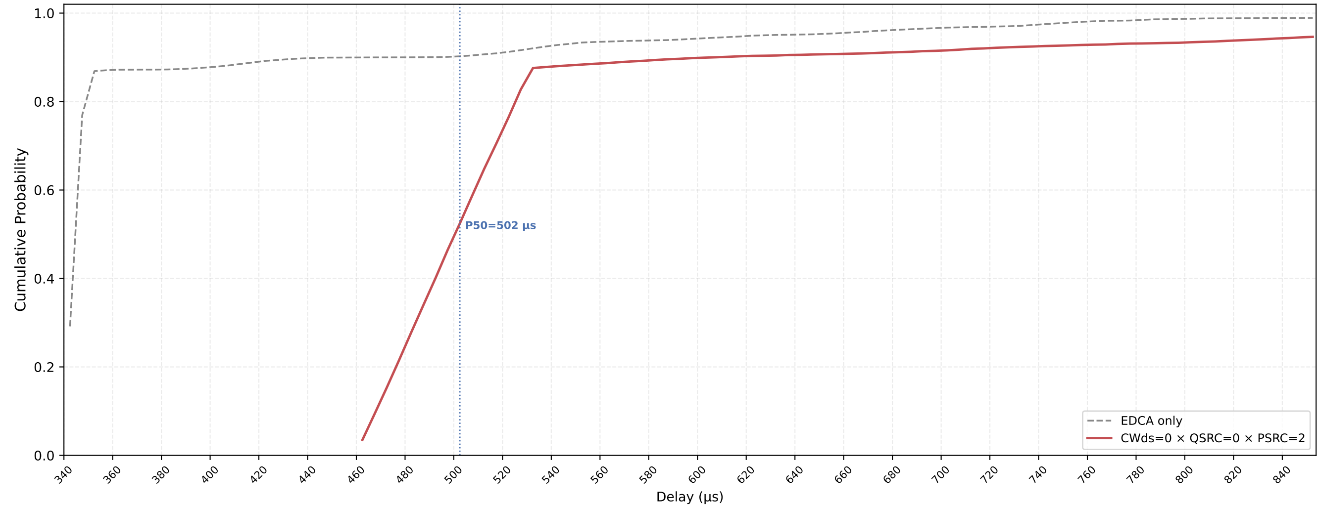
P-EDCA STA VO Delay CDF — CWds=0 × QSRC=0 × PSRC=2 nSta=30, nPedca=15, 0.1Mbps, avg of 10 runs
