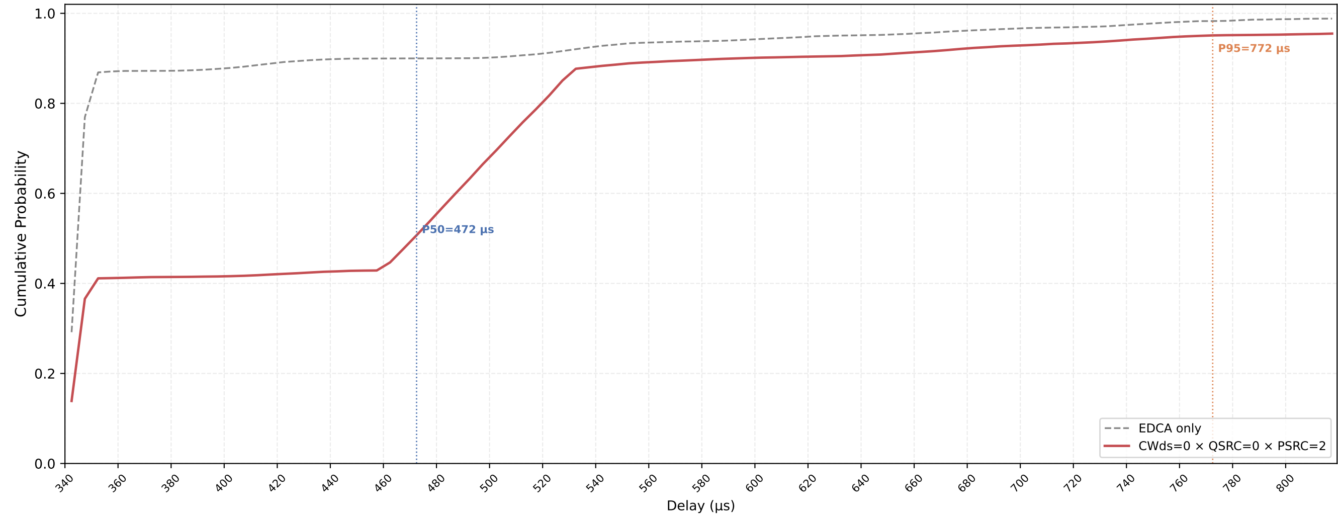
VO (all STAs) Delay CDF — CWds=0 × QSRC=0 × PSRC=2 nSta=30, nPedca=15, 0.1Mbps, avg of 10 runs
