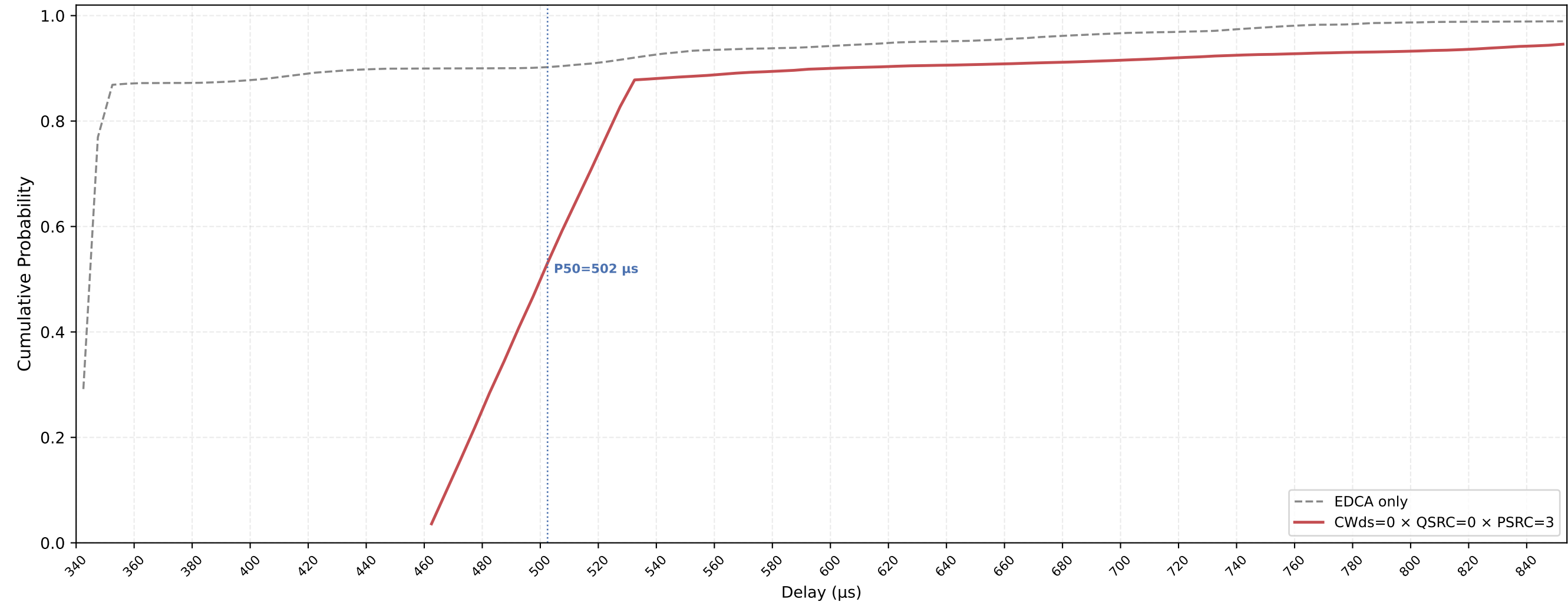
P-EDCA STA VO Delay CDF — CWds=0 × QSRC=0 × PSRC=3 nSta=30, nPedca=15, 0.1Mbps, avg of 10 runs
