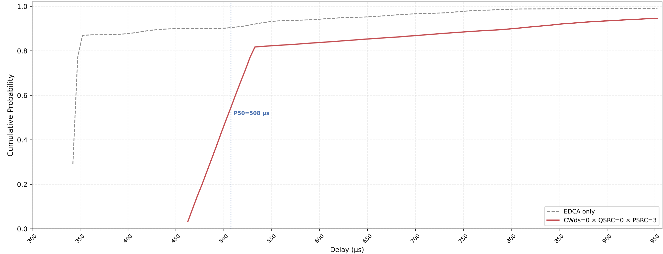
VO (all STAs) Delay CDF — CWds=0 × QSRC=0 × PSRC=3 nSta=30, nPedca=30, 0.1Mbps, avg of 10 runs
