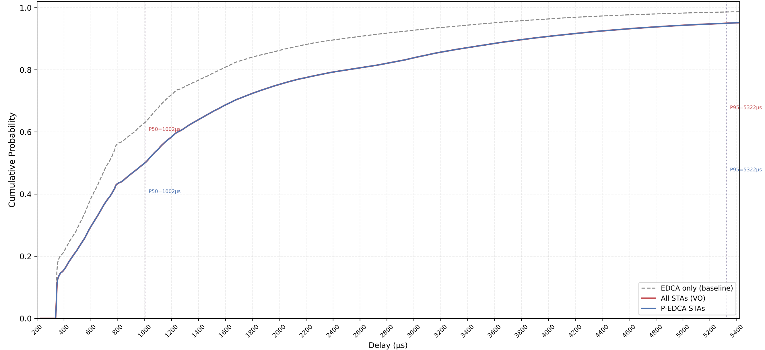
VO Delay CDF — P-EDCA / Legacy / All | CWds=0 × QSRC=1 × PSRC=1 nSta=30, nPedca=30/30, 0.5Mbps, avg of 10 runs
