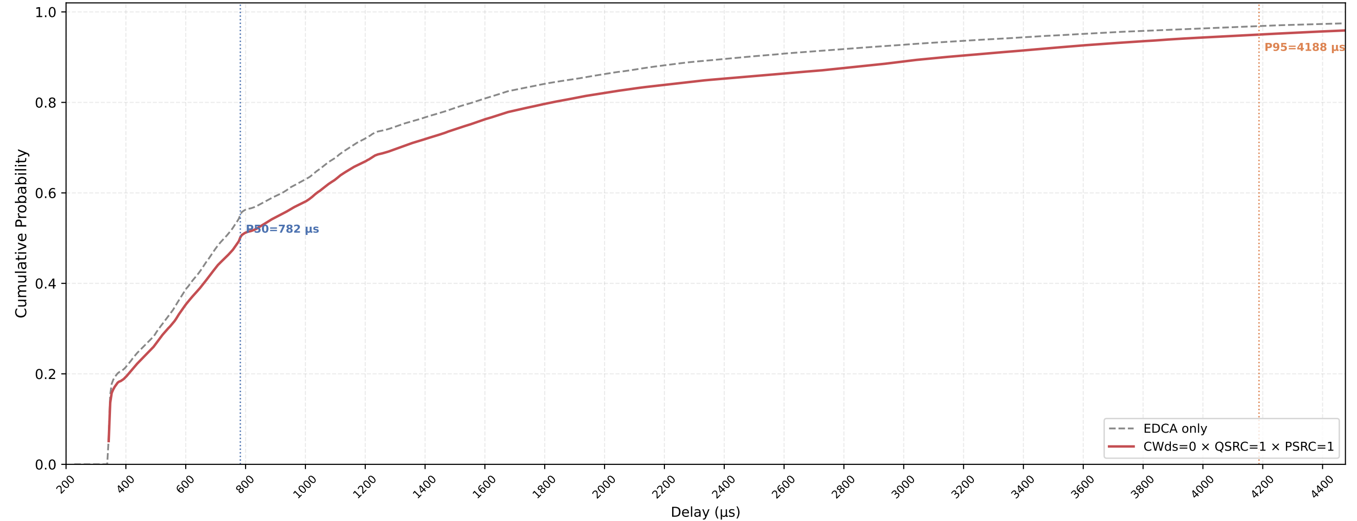
VO (all STAs) Delay CDF — CWds=0 × QSRC=1 × PSRC=1 nSta=30, nPedca=15, 0.5Mbps, avg of 10 runs
