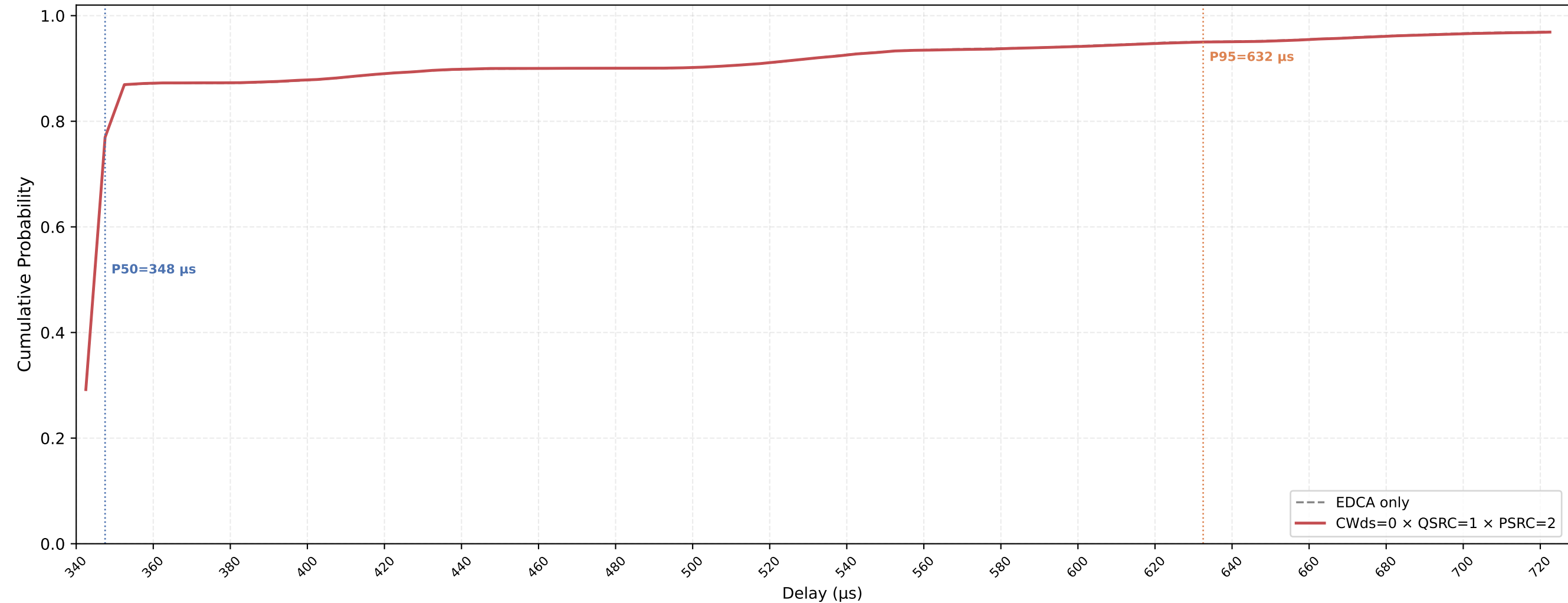
VO (all STAs) Delay CDF — CWds=0 × QSRC=1 × PSRC=2 nSta=30, nPedca=15, 0.1Mbps, avg of 10 runs
