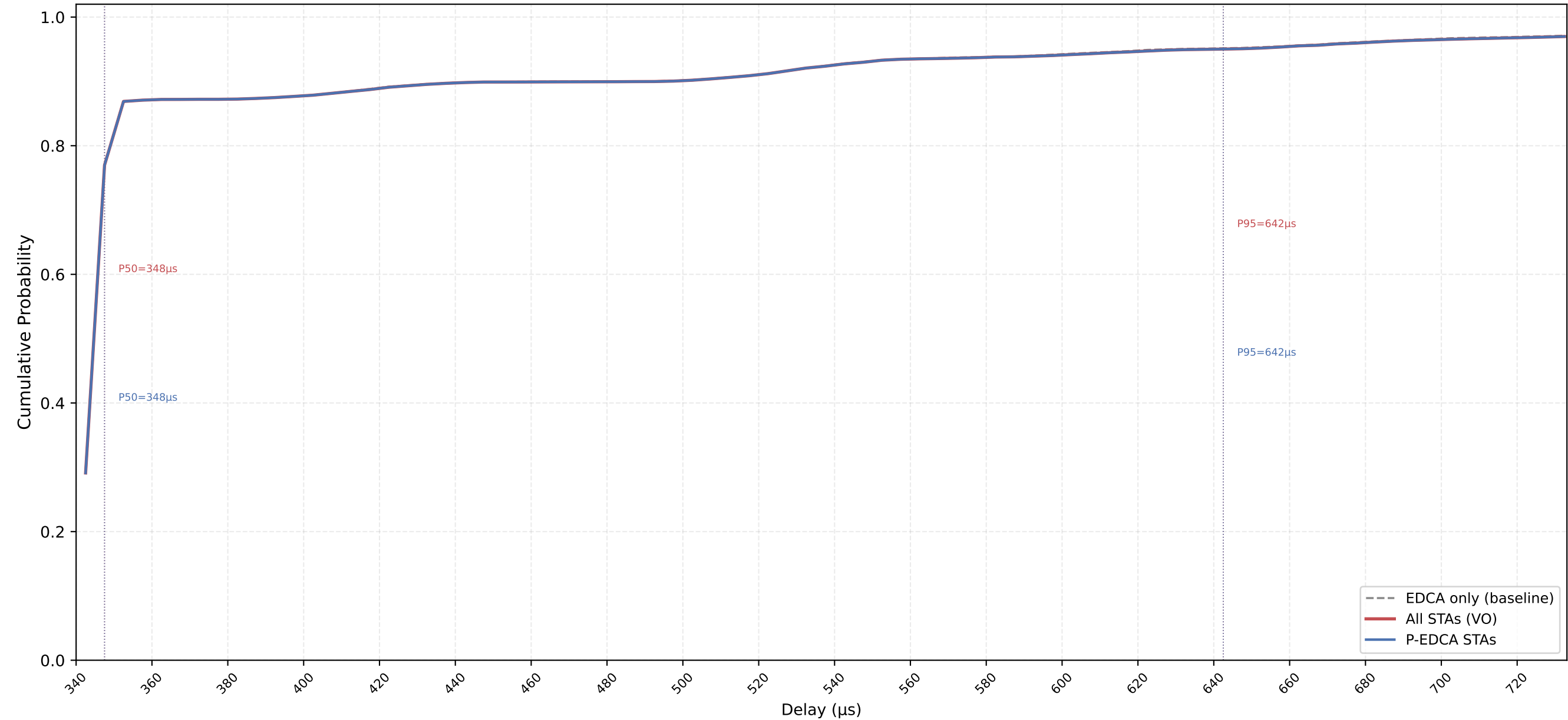
VO Delay CDF — P-EDCA / Legacy / All | CWds=0 × QSRC=1 × PSRC=3 nSta=30, nPedca=30/30, 0.1Mbps, avg of 10 runs
