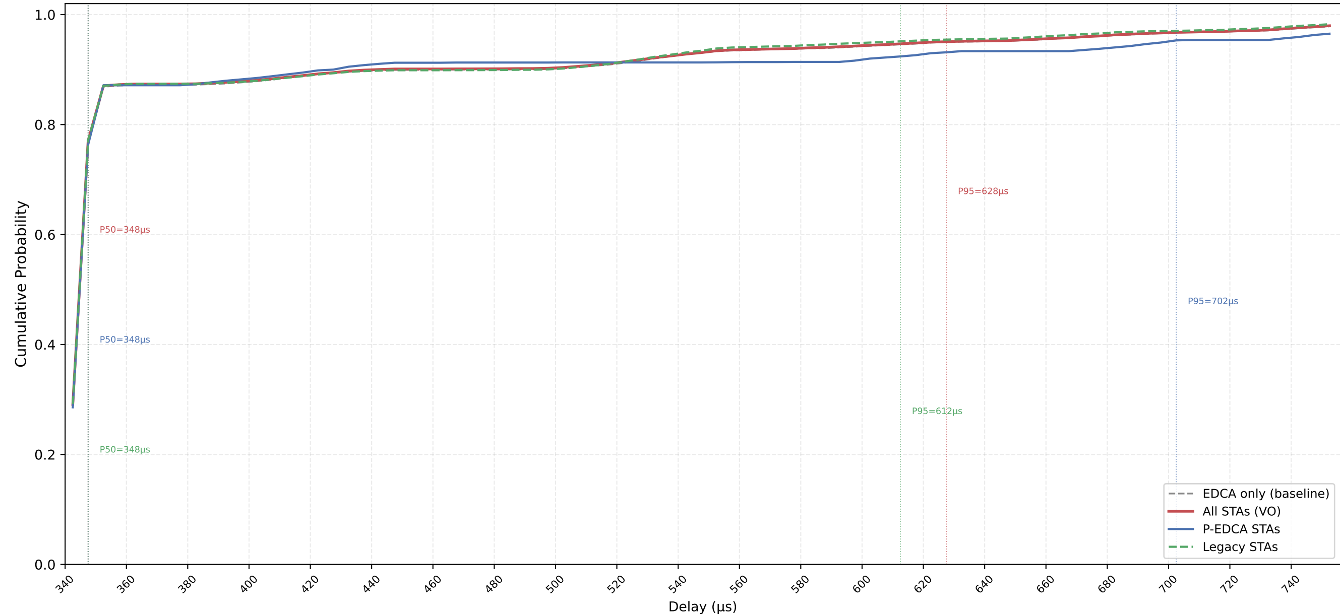
VO Delay CDF — P-EDCA / Legacy / All | CWds=0 × QSRC=2 × PSRC=2 nSta=30, nPedca=5/30, 0.1Mbps, avg of 10 runs
