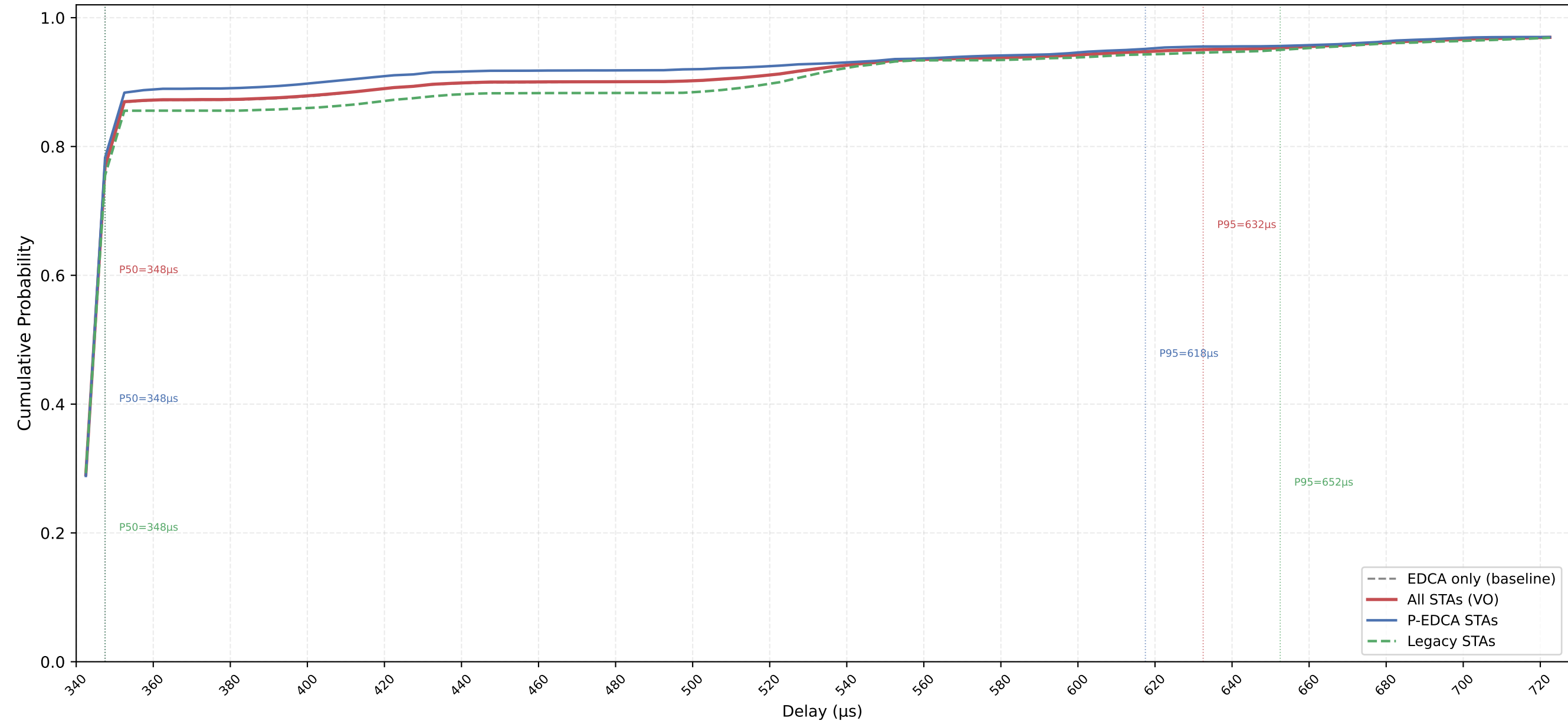
VO Delay CDF — P-EDCA / Legacy / All | CWds=0 × QSRC=2 × PSRC=2 nSta=30, nPedca=15/30, 0.1Mbps, avg of 10 runs
