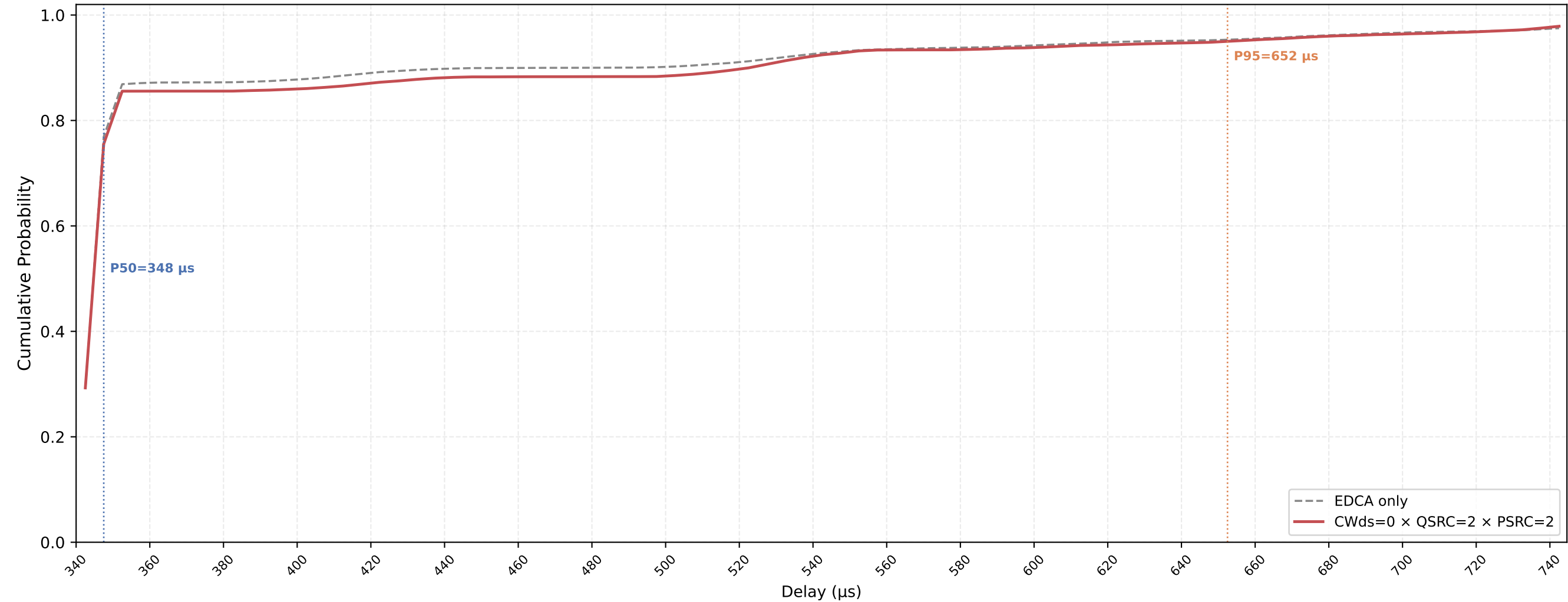
Legacy STA VO Delay CDF — CWds=0 × QSRC=2 × PSRC=2 nSta=30, nPedca=15, 0.1Mbps, avg of 10 runs
