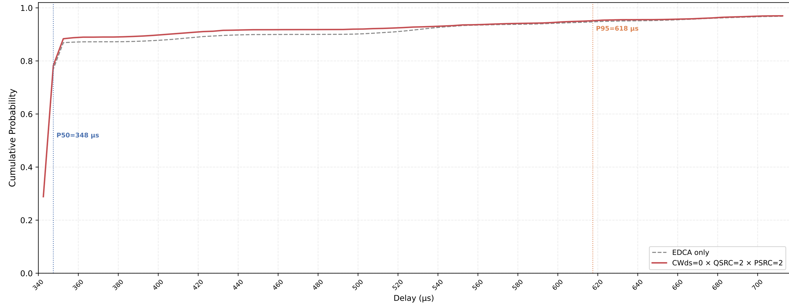
P-EDCA STA VO Delay CDF — CWds=0 × QSRC=2 × PSRC=2 nSta=30, nPedca=15, 0.1Mbps, avg of 10 runs
