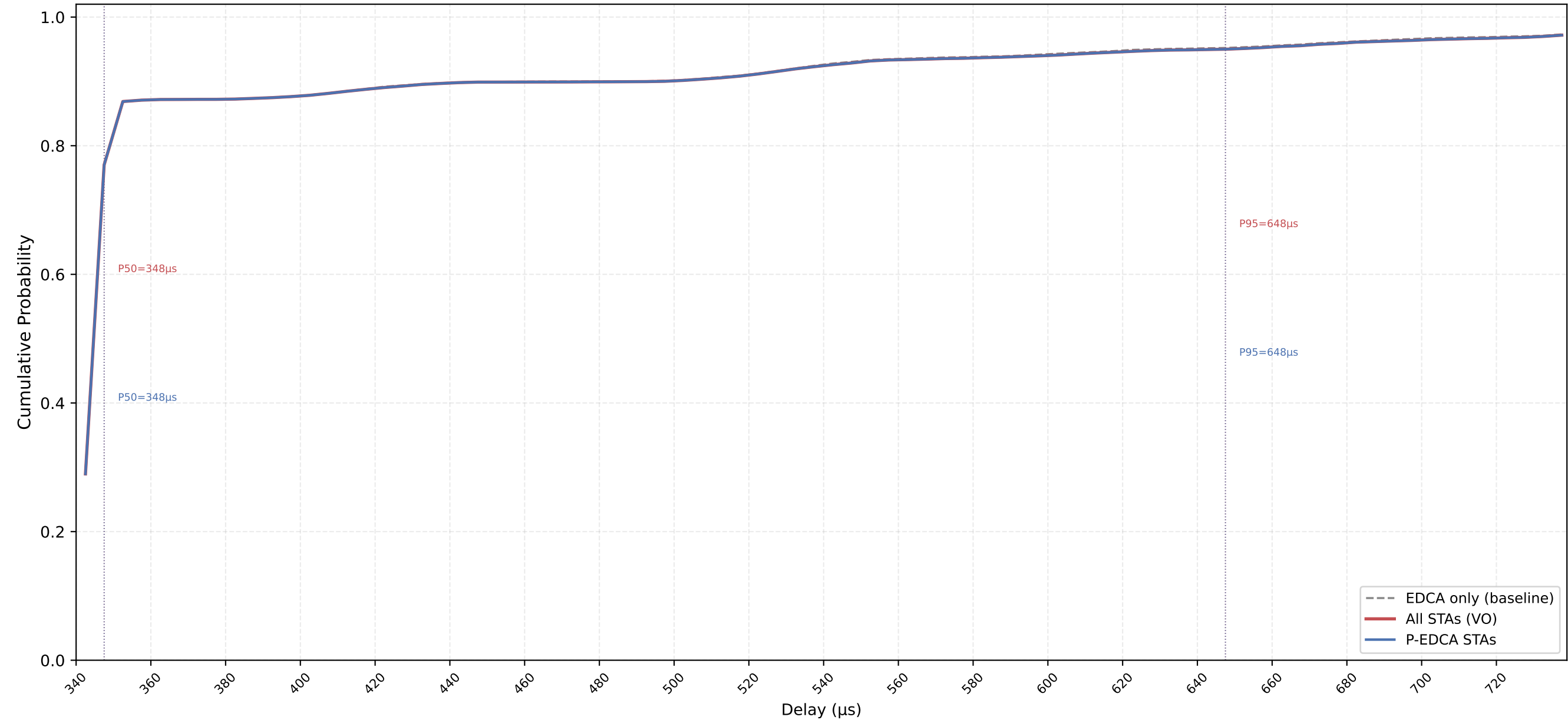
VO Delay CDF — P-EDCA / Legacy / All | CWds=0 × QSRC=2 × PSRC=3 nSta=30, nPedca=30/30, 0.1Mbps, avg of 10 runs
