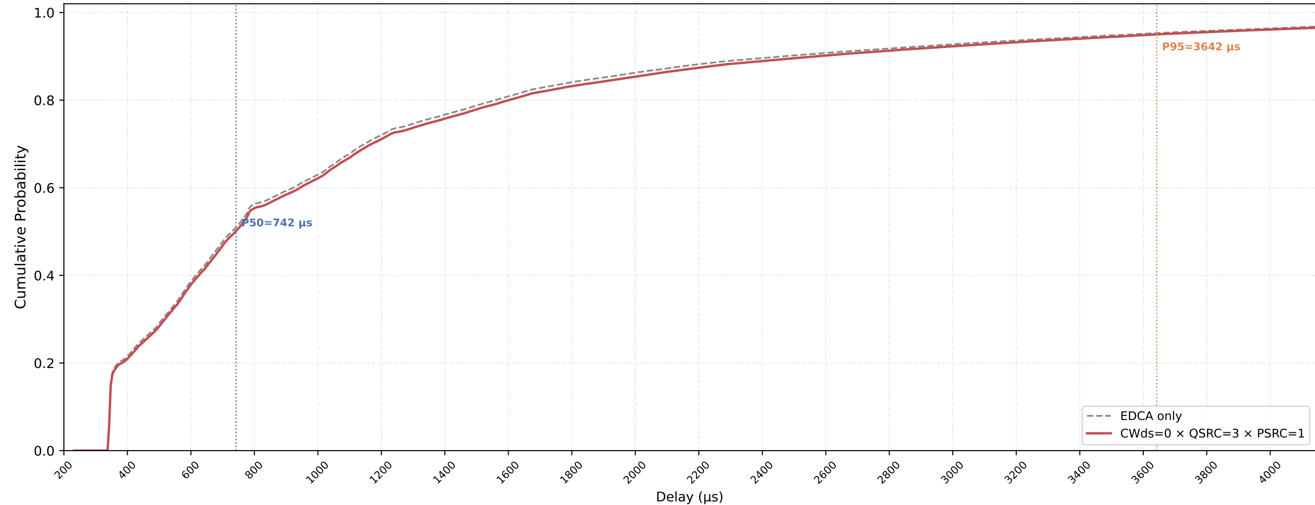
VO (all STAs) Delay CDF — CWds=0 × QSRC=3 × PSRC=1 nSta=30, nPedca=15, 0.5Mbps, avg of 10 runs
