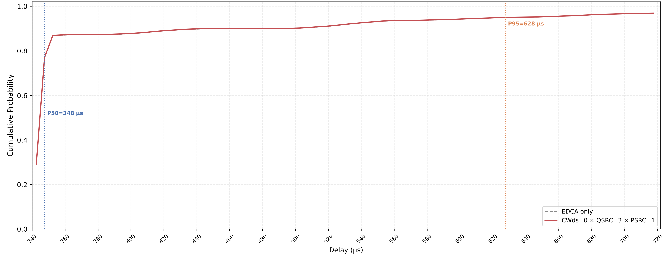
VO (all STAs) Delay CDF — CWds=0 × QSRC=3 × PSRC=1 nSta=30, nPedca=30, 0.1Mbps, avg of 10 runs
