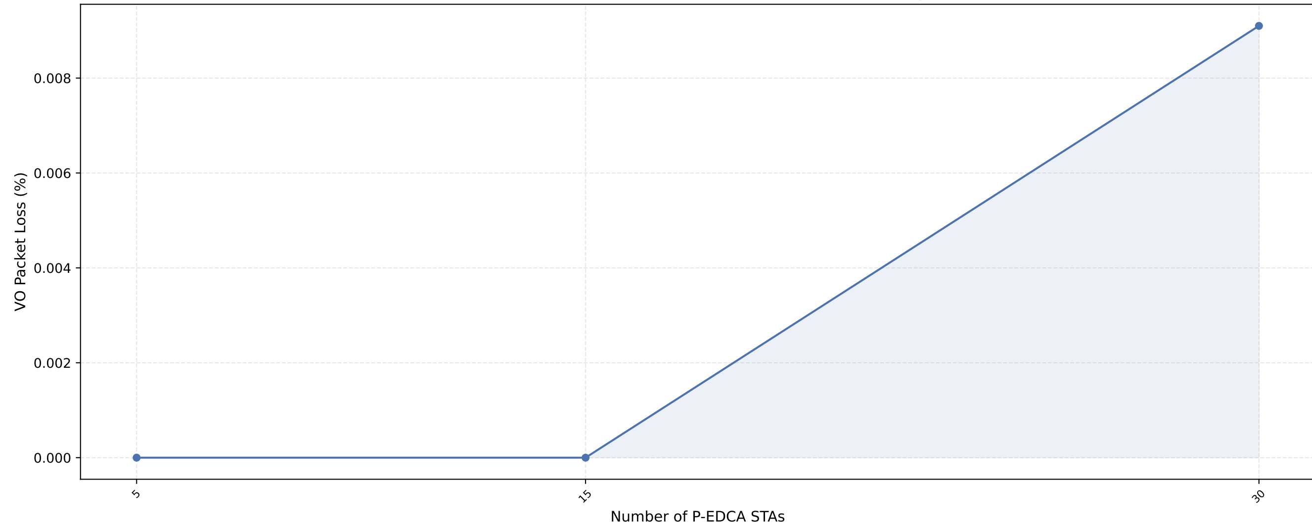
VO Packet Loss vs P-EDCA STAs — nSta=30, 0.1Mbps (avg of 10 runs)
