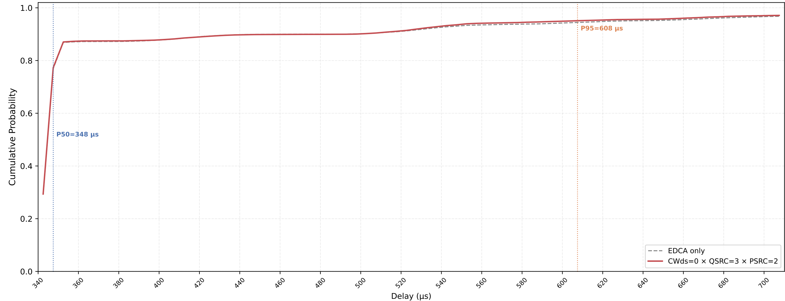
Legacy STA VO Delay CDF — CWds=0 × QSRC=3 × PSRC=2 nSta=30, nPedca=5, 0.1Mbps, avg of 10 runs
