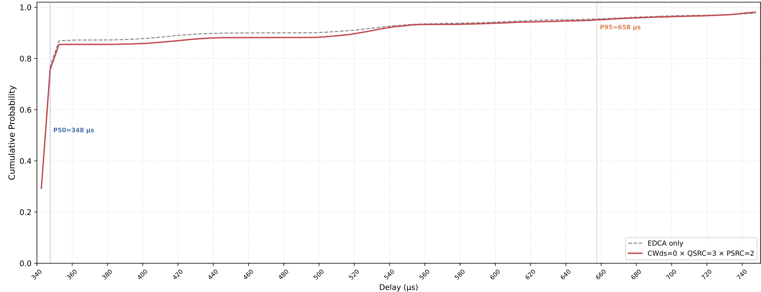
Legacy STA VO Delay CDF — CWds=0 × QSRC=3 × PSRC=2 nSta=30, nPedca=15, 0.1Mbps, avg of 10 runs
