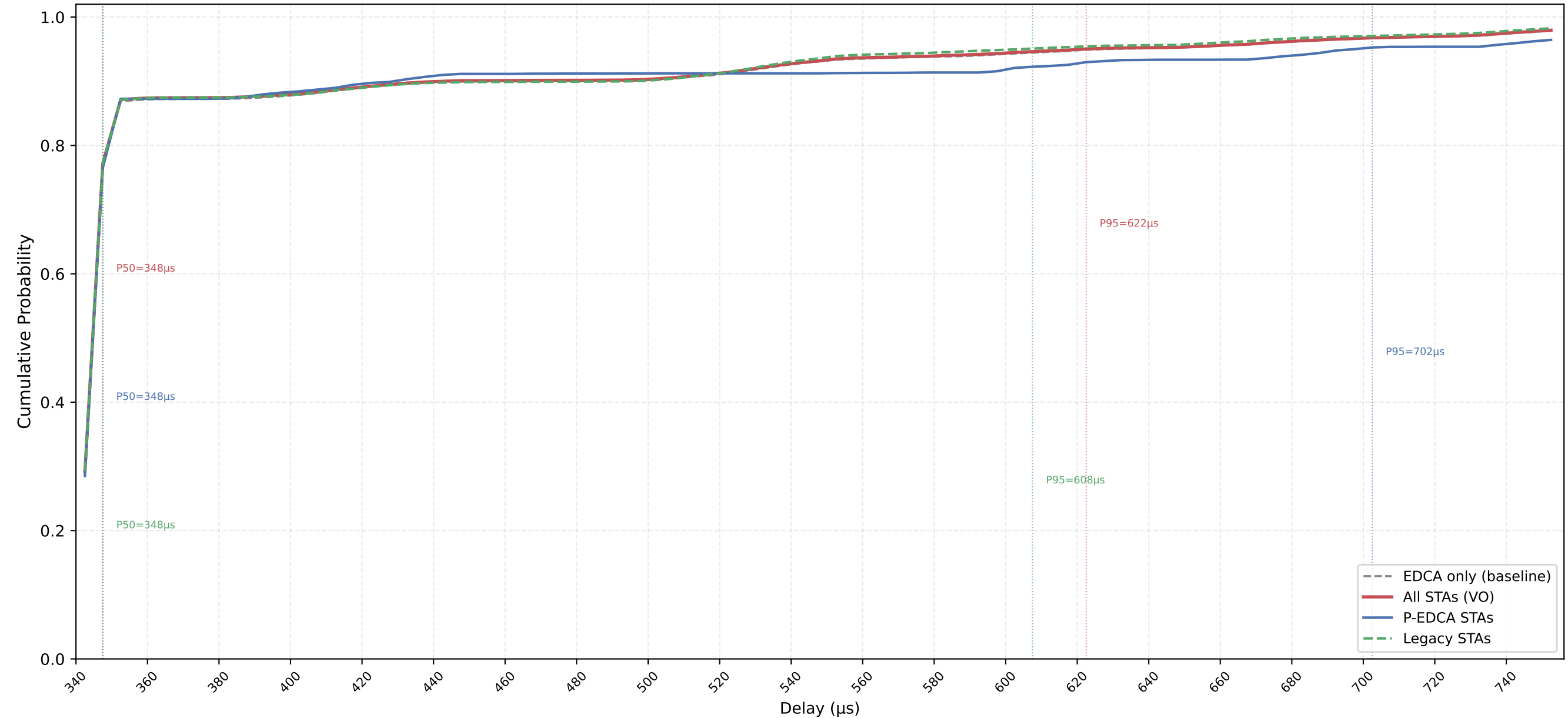
VO Delay CDF — P-EDCA / Legacy / All | CWds=0 × QSRC=3 × PSRC=3 nSta=30, nPedca=5/30, 0.1Mbps, avg of 10 runs
