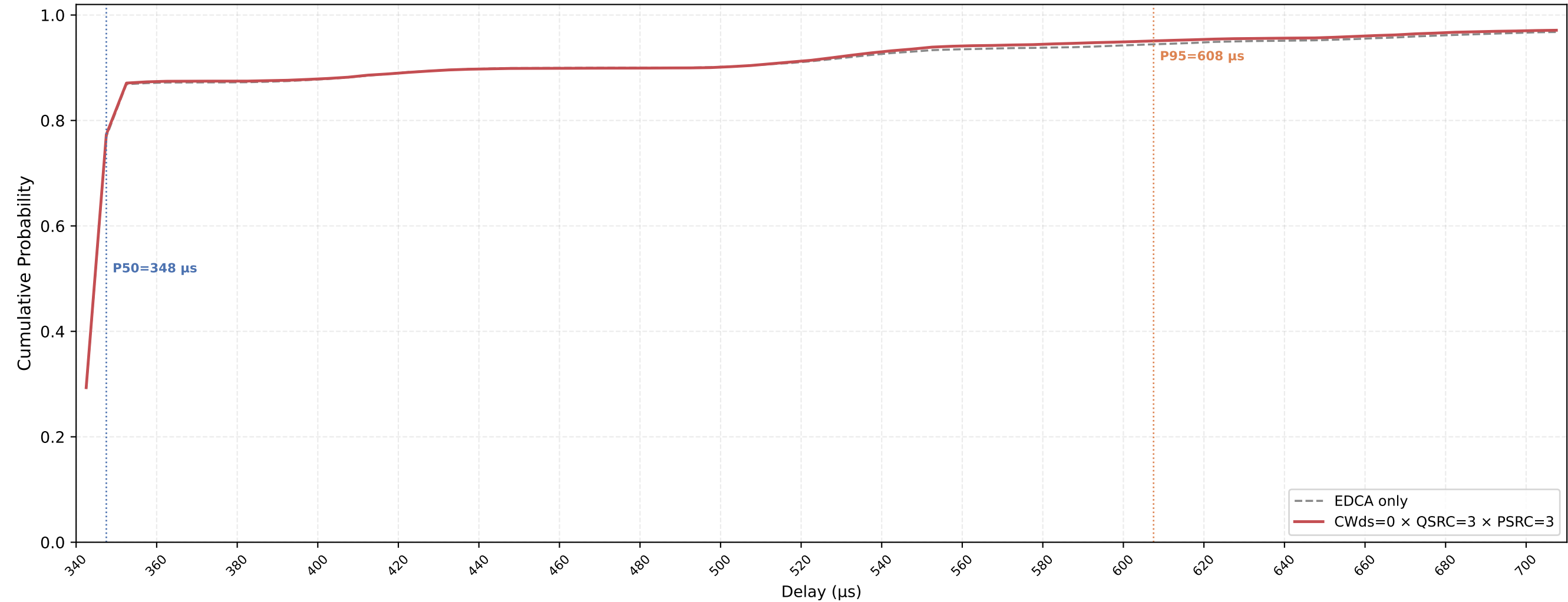
Legacy STA VO Delay CDF — CWds=0 × QSRC=3 × PSRC=3 nSta=30, nPedca=5, 0.1Mbps, avg of 10 runs
