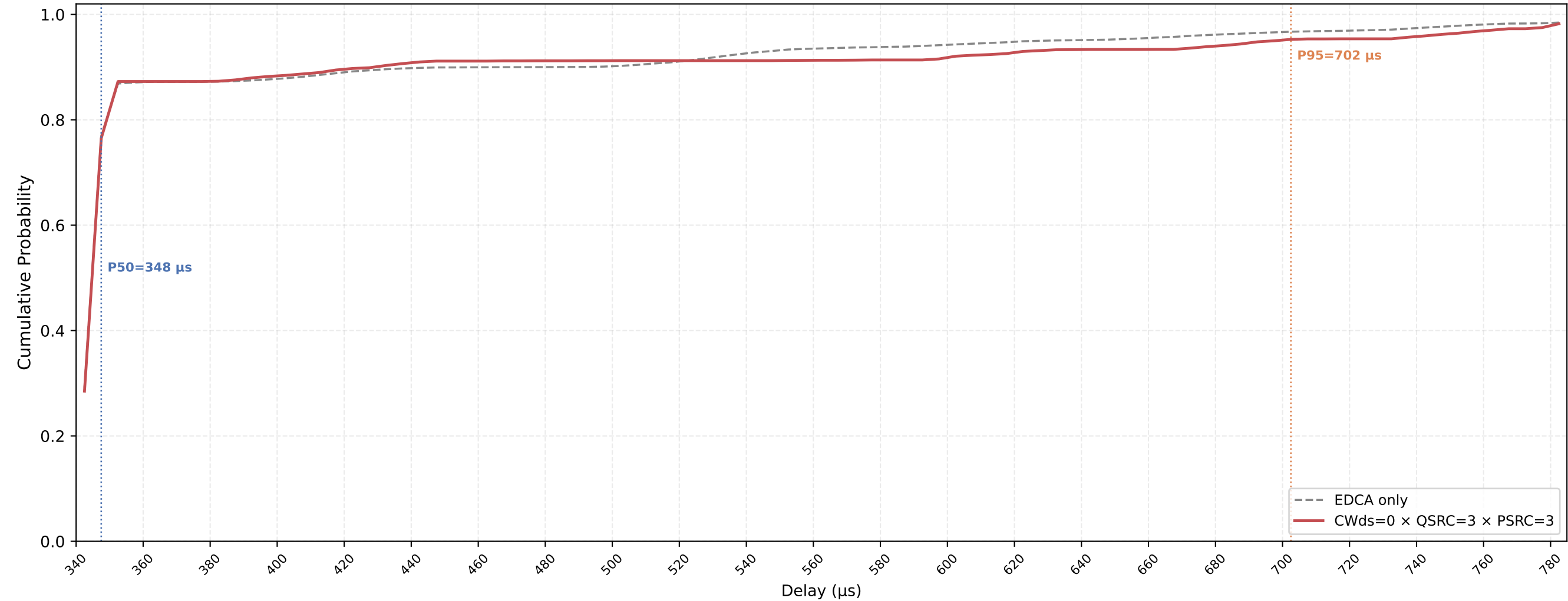
P-EDCA STA VO Delay CDF — CWds=0 × QSRC=3 × PSRC=3 nSta=30, nPedca=5, 0.1Mbps, avg of 10 runs
