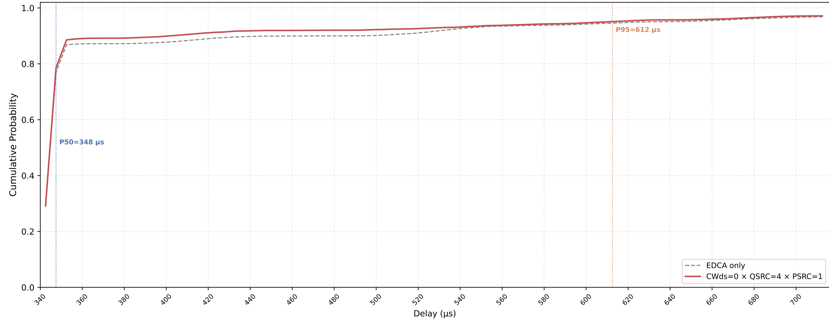
P-EDCA STA VO Delay CDF — CWds=0 × QSRC=4 × PSRC=1 nSta=30, nPedca=15, 0.1Mbps, avg of 10 runs
