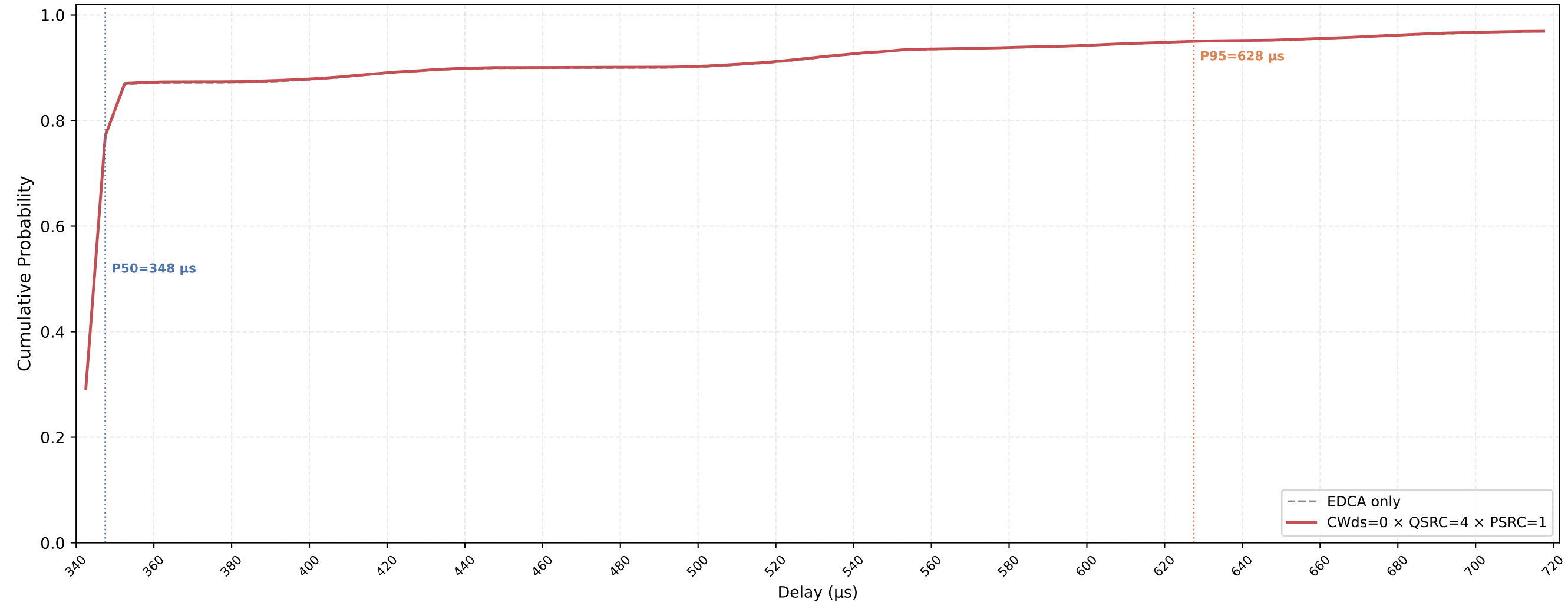
VO (all STAs) Delay CDF — CWds=0 × QSRC=4 × PSRC=1 nSta=30, nPedca=15, 0.1Mbps, avg of 10 runs
