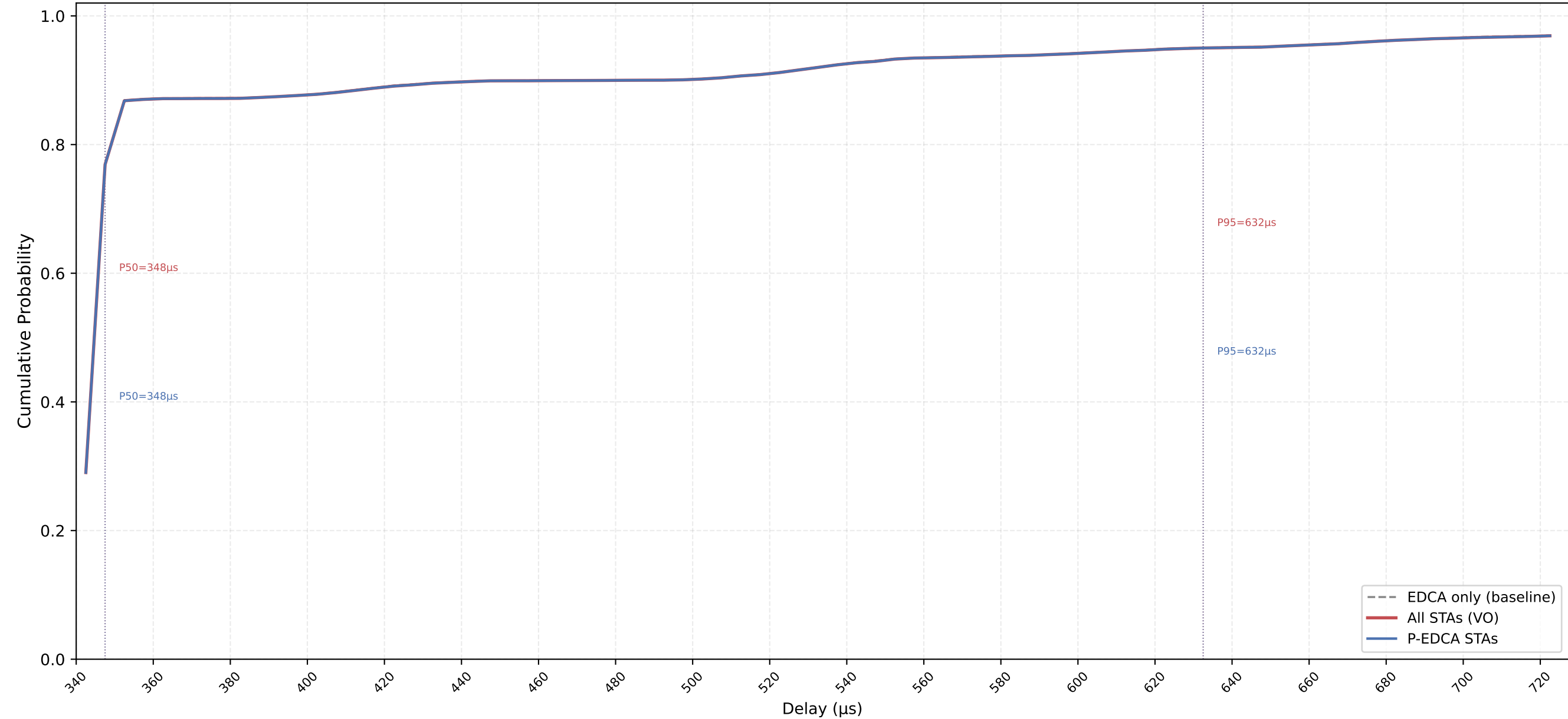
VO Delay CDF — P-EDCA / Legacy / All | CWds=0 × QSRC=4 × PSRC=3 nSta=30, nPedca=30/30, 0.1Mbps, avg of 10 runs
