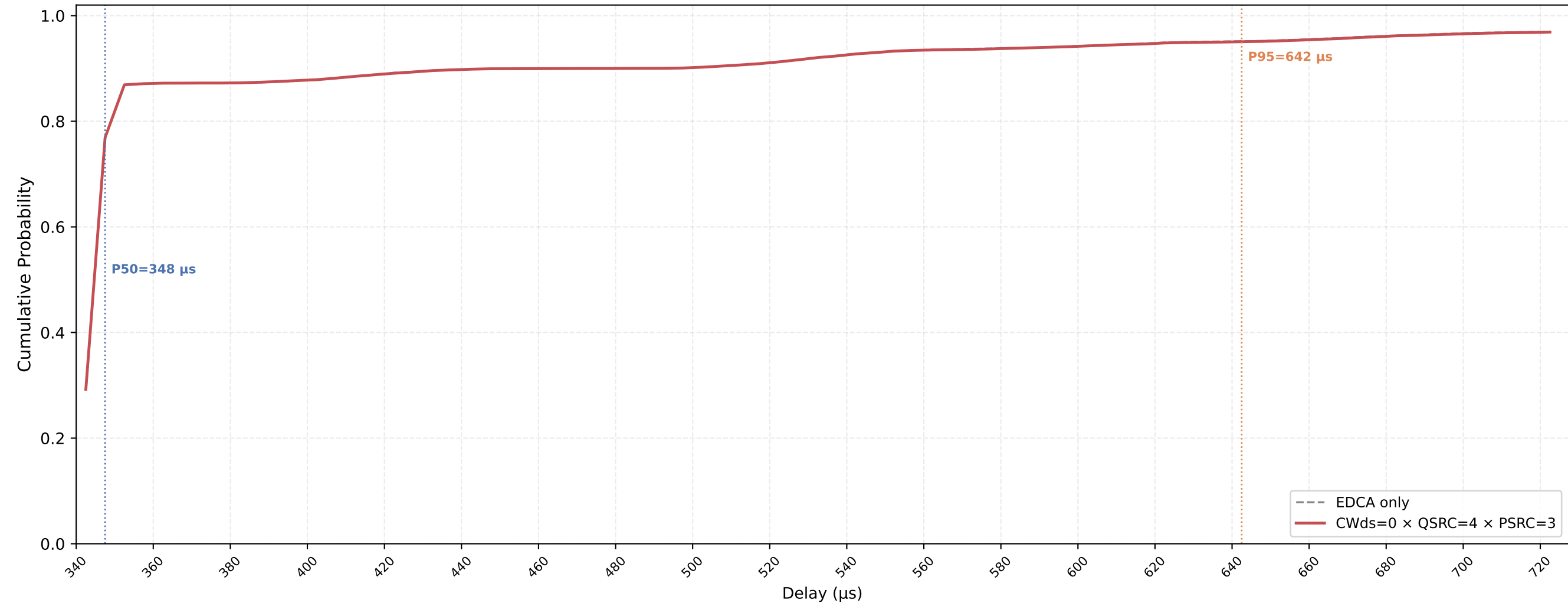
VO (all STAs) Delay CDF — CWds=0 × QSRC=4 × PSRC=3 nSta=30, nPedca=15, 0.1Mbps, avg of 10 runs
