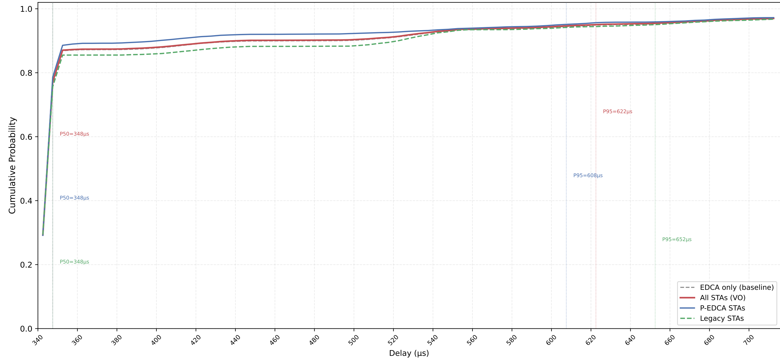
VO Delay CDF — P-EDCA / Legacy / All | CWds=0 × QSRC=5 × PSRC=1 nSta=30, nPedca=15/30, 0.1Mbps, avg of 10 runs
