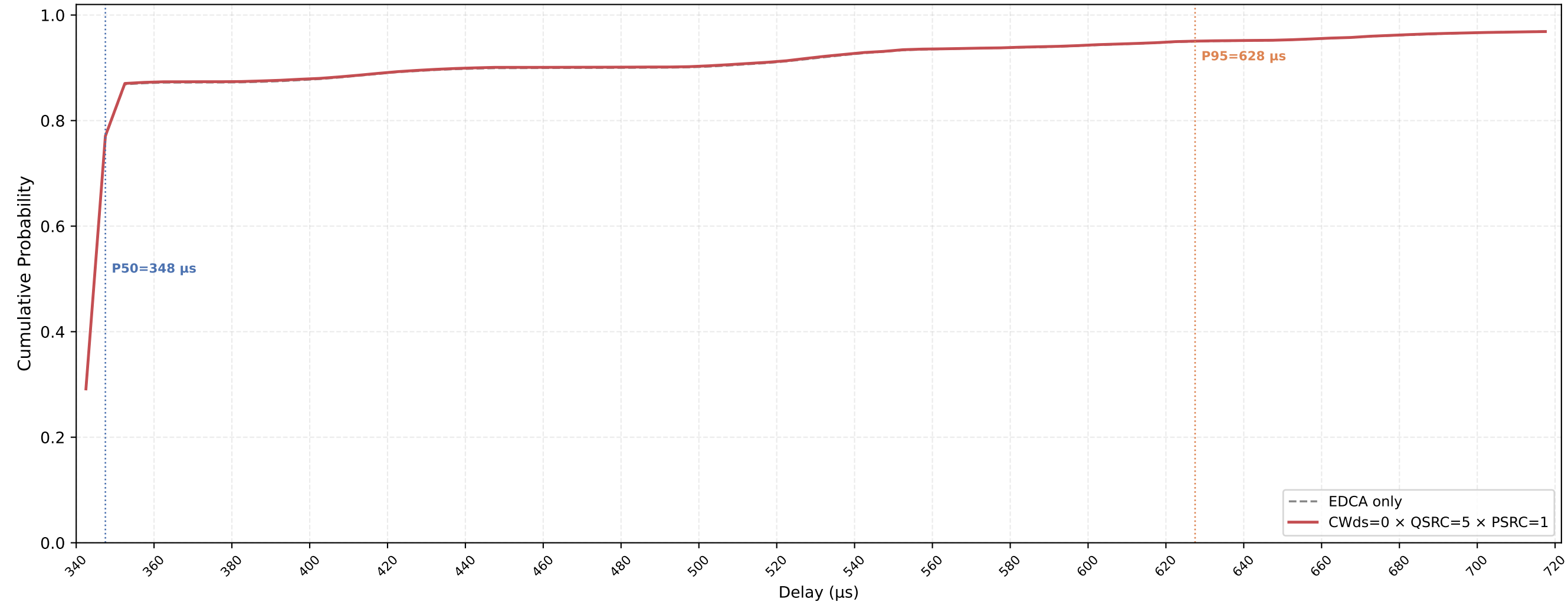
VO (all STAs) Delay CDF — CWds=0 × QSRC=5 × PSRC=1 nSta=30, nPedca=5, 0.1Mbps, avg of 10 runs
