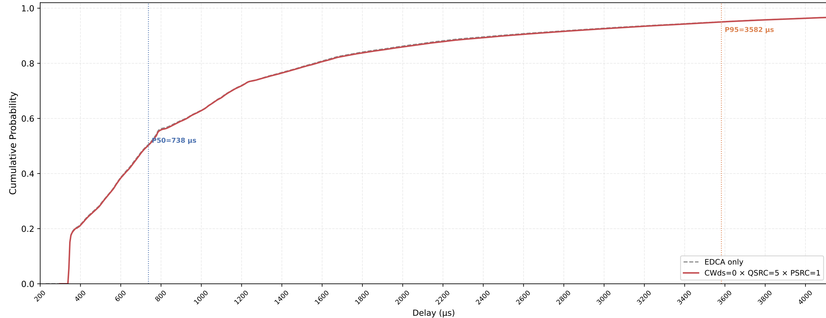
VO (all STAs) Delay CDF — CWds=0 × QSRC=5 × PSRC=1 nSta=30, nPedca=5, 0.5Mbps, avg of 10 runs
