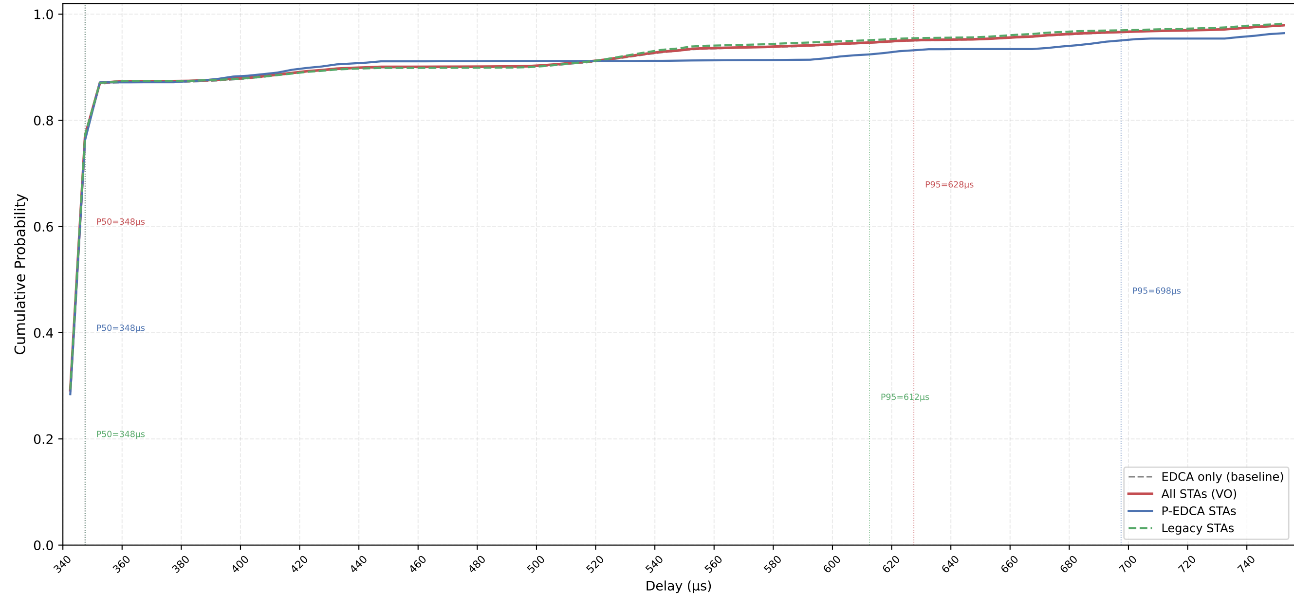
VO Delay CDF — P-EDCA / Legacy / All | CWds=0 × QSRC=5 × PSRC=2 nSta=30, nPedca=5/30, 0.1Mbps, avg of 10 runs
