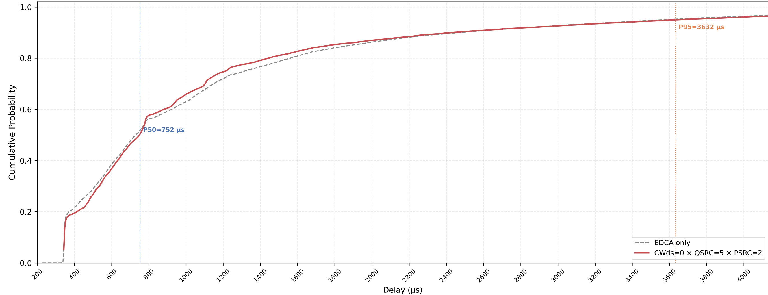
P-EDCA STA VO Delay CDF — CWds=0 × QSRC=5 × PSRC=2 nSta=30, nPedca=5, 0.5Mbps, avg of 10 runs
