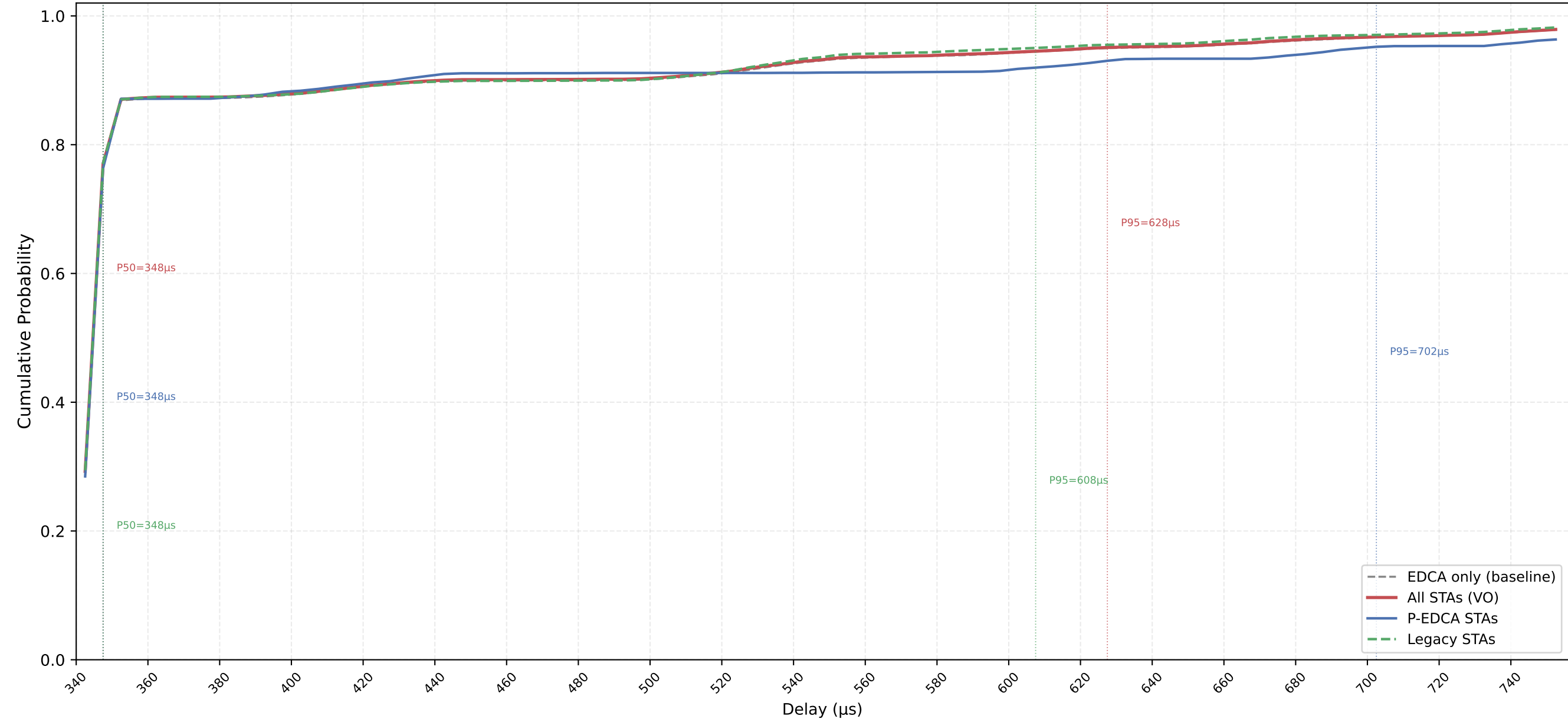
VO Delay CDF — P-EDCA / Legacy / All | CWds=0 × QSRC=5 × PSRC=3 nSta=30, nPedca=5/30, 0.1Mbps, avg of 10 runs
