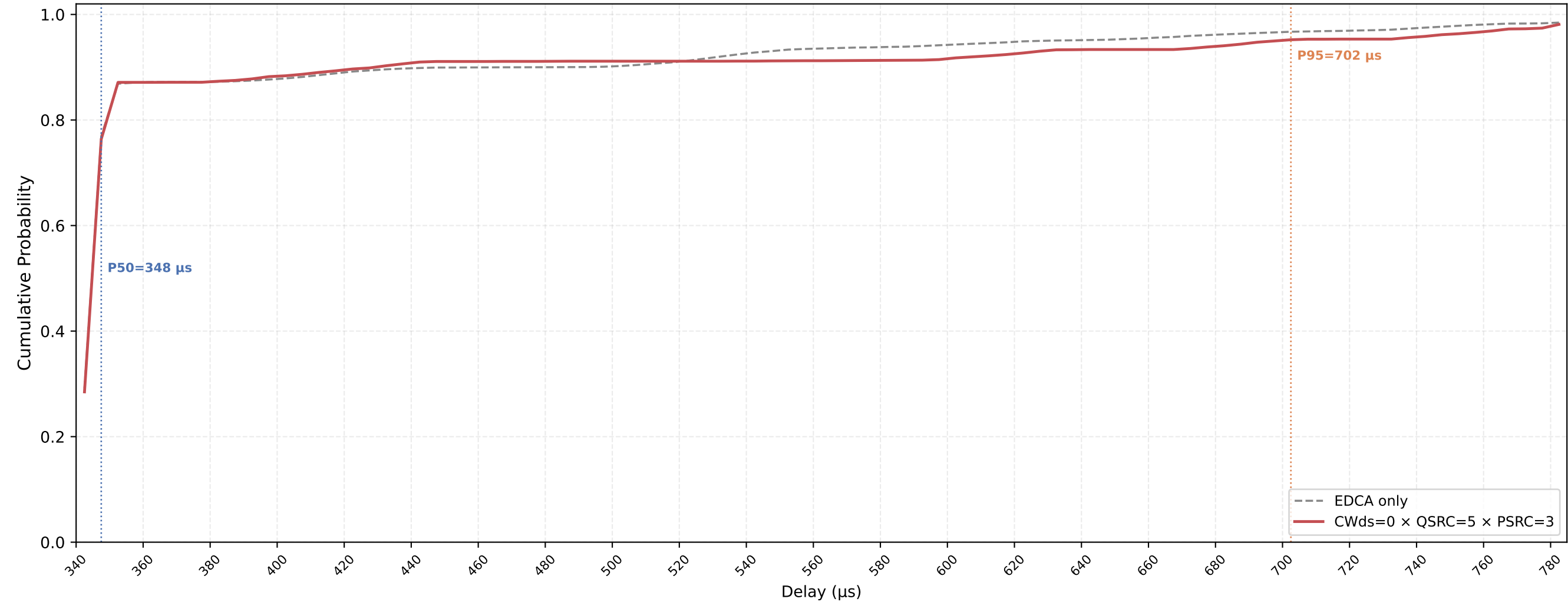
P-EDCA STA VO Delay CDF — CWds=0 × QSRC=5 × PSRC=3 nSta=30, nPedca=5, 0.1Mbps, avg of 10 runs
