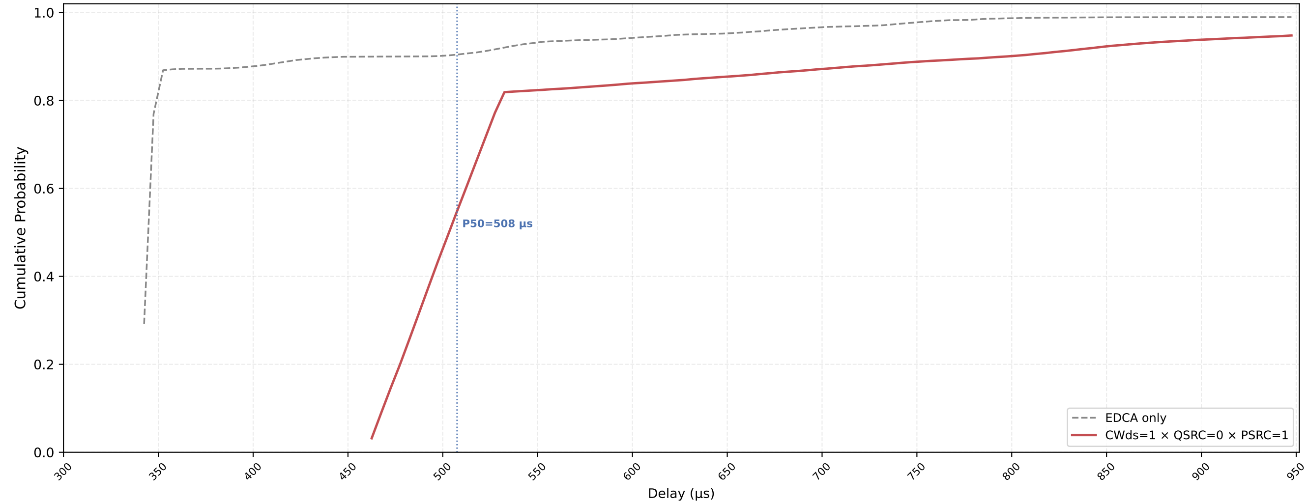
VO (all STAs) Delay CDF — CWds=1 × QSRC=0 × PSRC=1 nSta=30, nPedca=30, 0.1Mbps, avg of 10 runs
