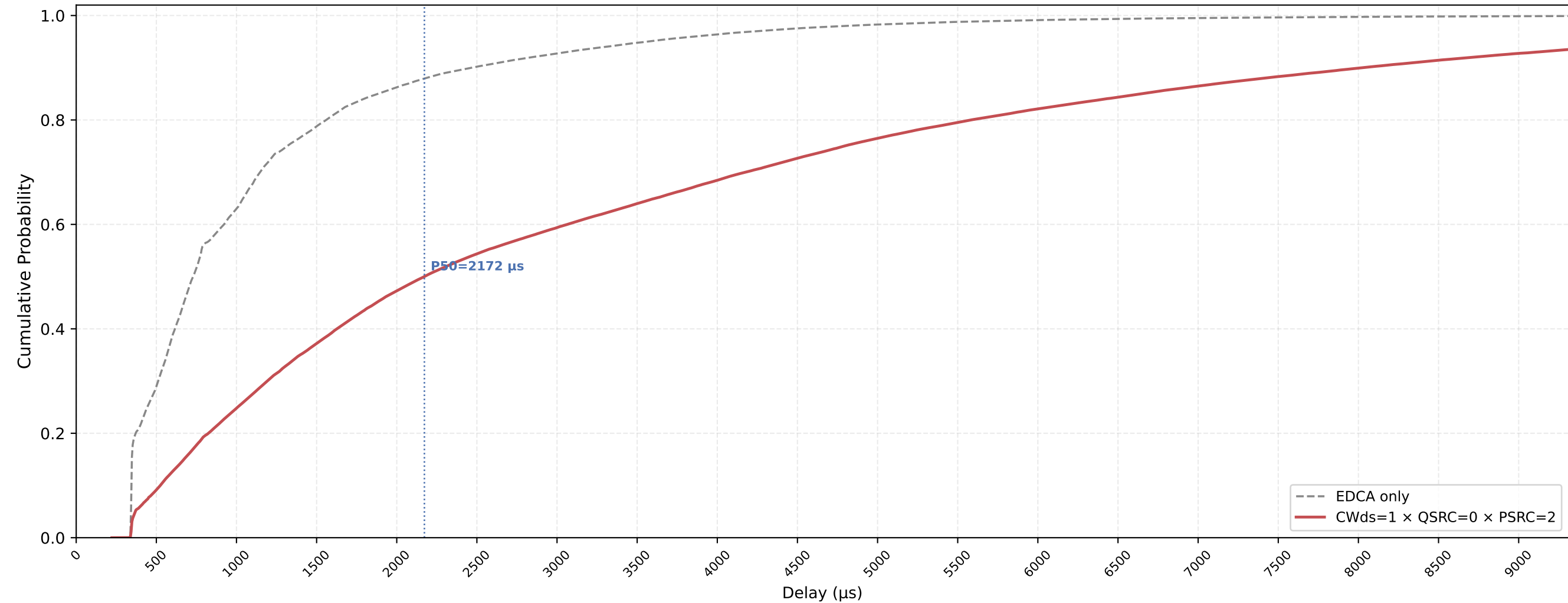
Legacy STA VO Delay CDF — CWds=1 × QSRC=0 × PSRC=2 nSta=30, nPedca=15, 0.5Mbps, avg of 10 runs
