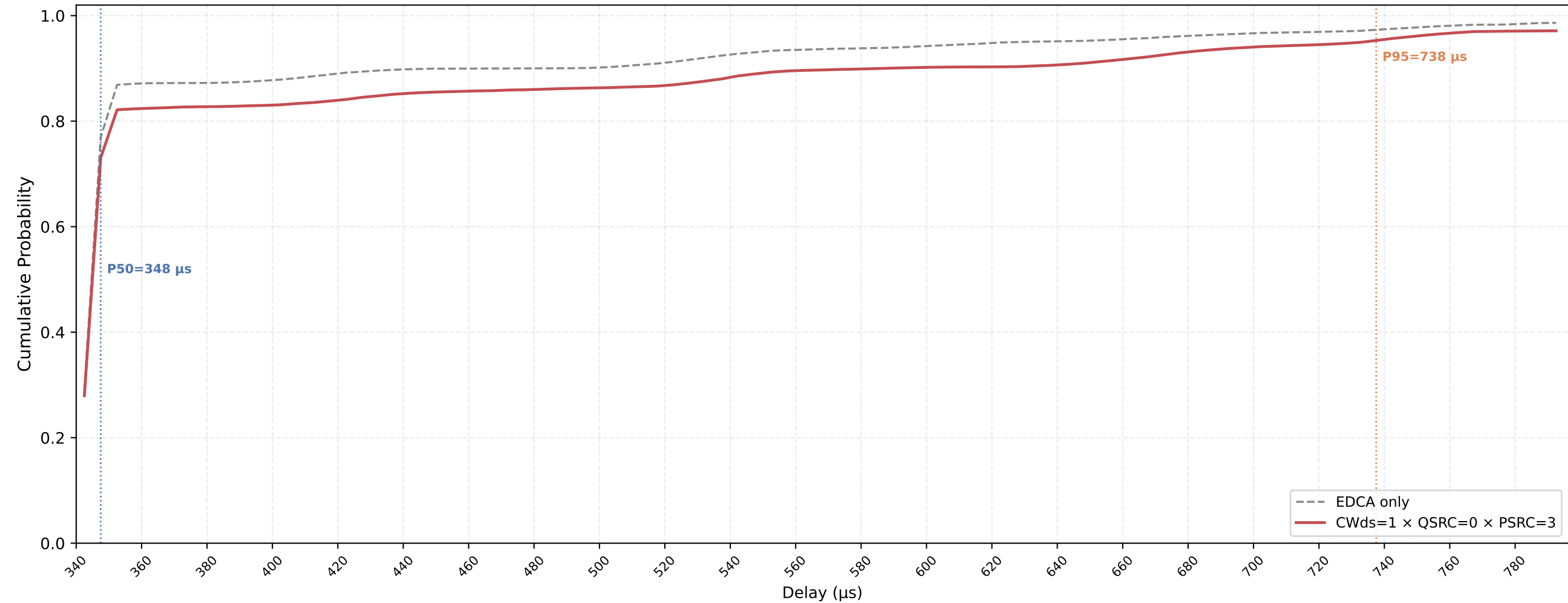
Legacy STA VO Delay CDF — CWds=1 × QSRC=0 × PSRC=3 nSta=30, nPedca=15, 0.1Mbps, avg of 10 runs
