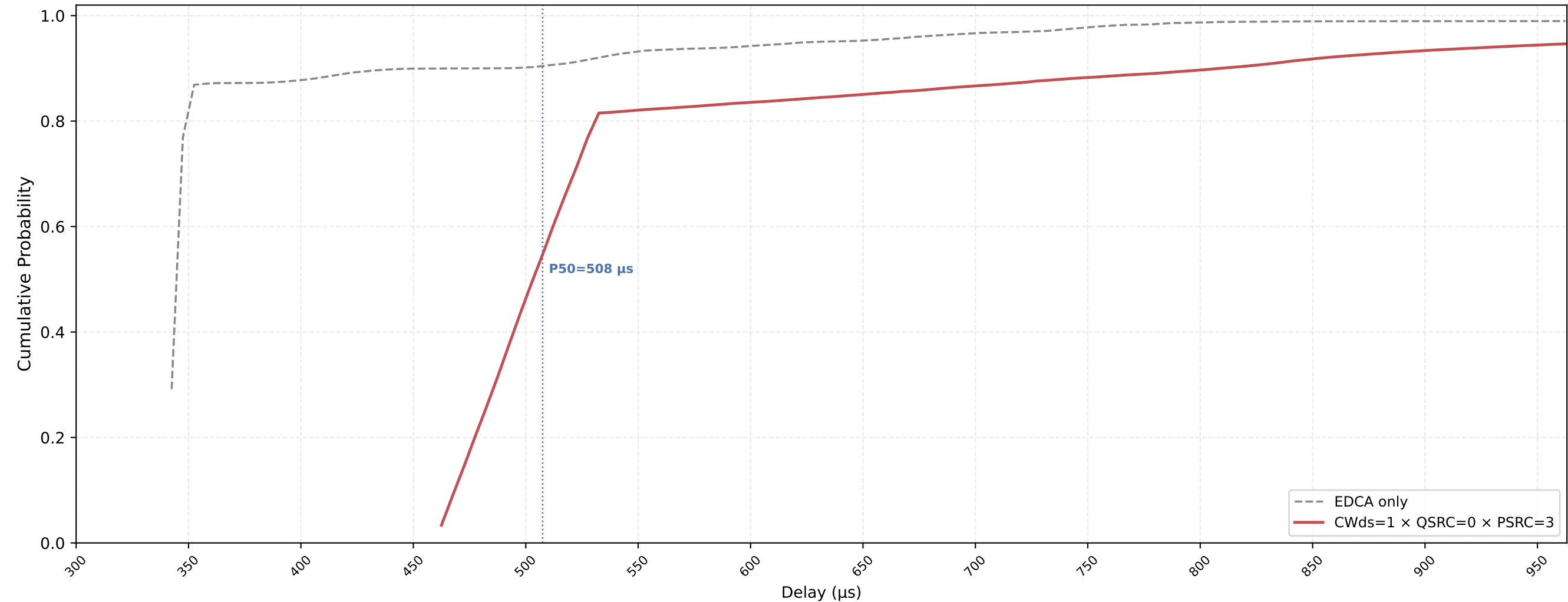
P-EDCA STA VO Delay CDF — CWds=1 × QSRC=0 × PSRC=3 nSta=30, nPedca=30, 0.1Mbps, avg of 10 runs
