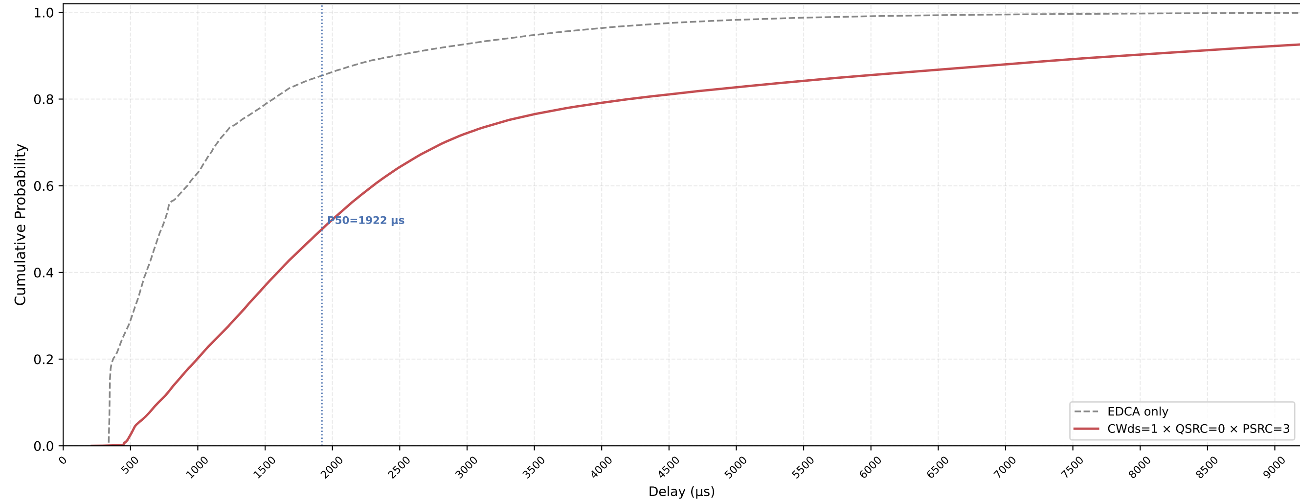
P-EDCA STA VO Delay CDF — CWds=1 × QSRC=0 × PSRC=3 nSta=30, nPedca=30, 0.5Mbps, avg of 10 runs
