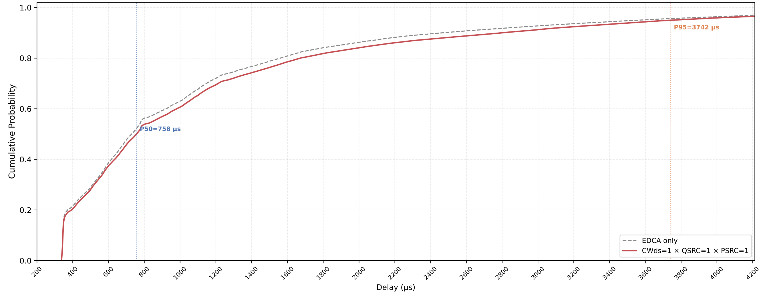
VO (all STAs) Delay CDF — CWds=1 × QSRC=1 × PSRC=1 nSta=30, nPedca=5, 0.5Mbps, avg of 10 runs
